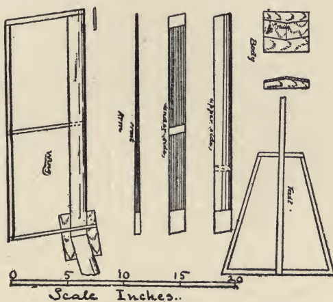
Other Parts of Huffaker's Bird Model.
