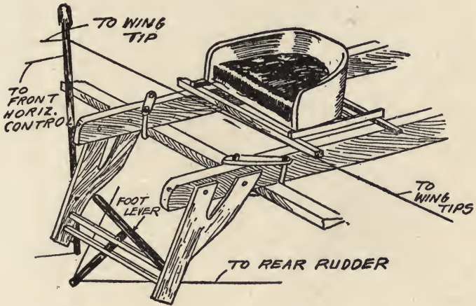
System of Control on Farman Machine.
