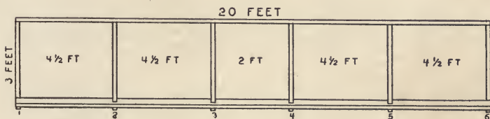
Framework of Glider With Struts in Place.
