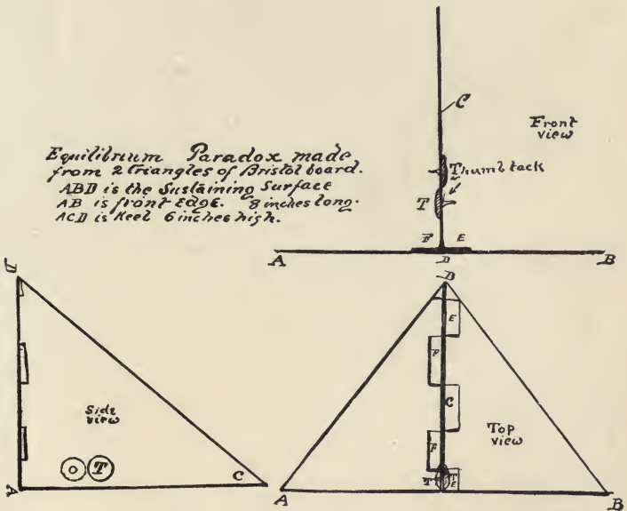
Equilibrium Paradox Explained.
