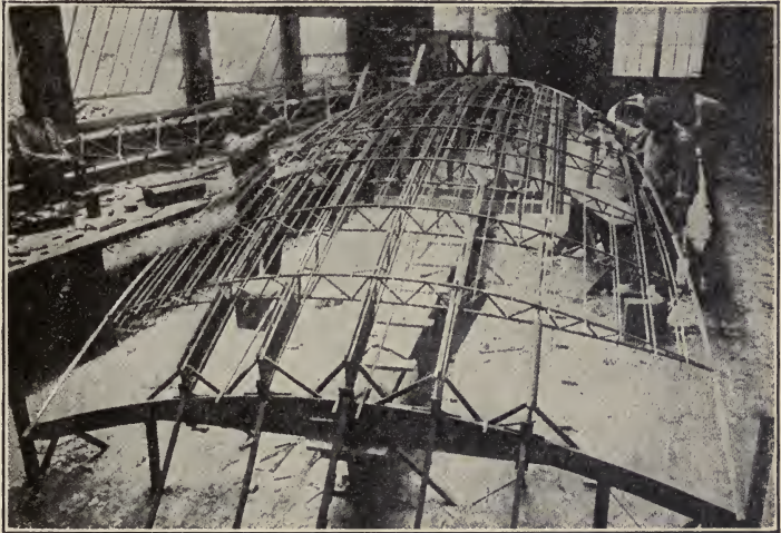
Framework of Bleriot Monoplane.
