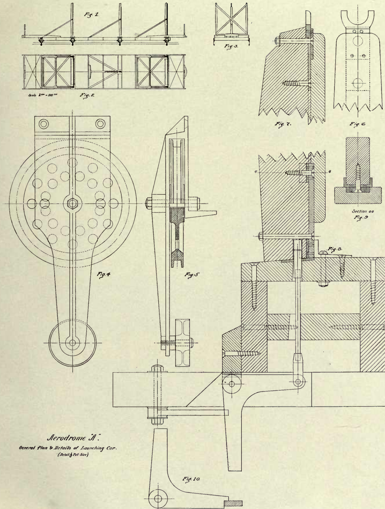
GENERAL PLAN AND DETAILS OF LAUNCHING-CAR
