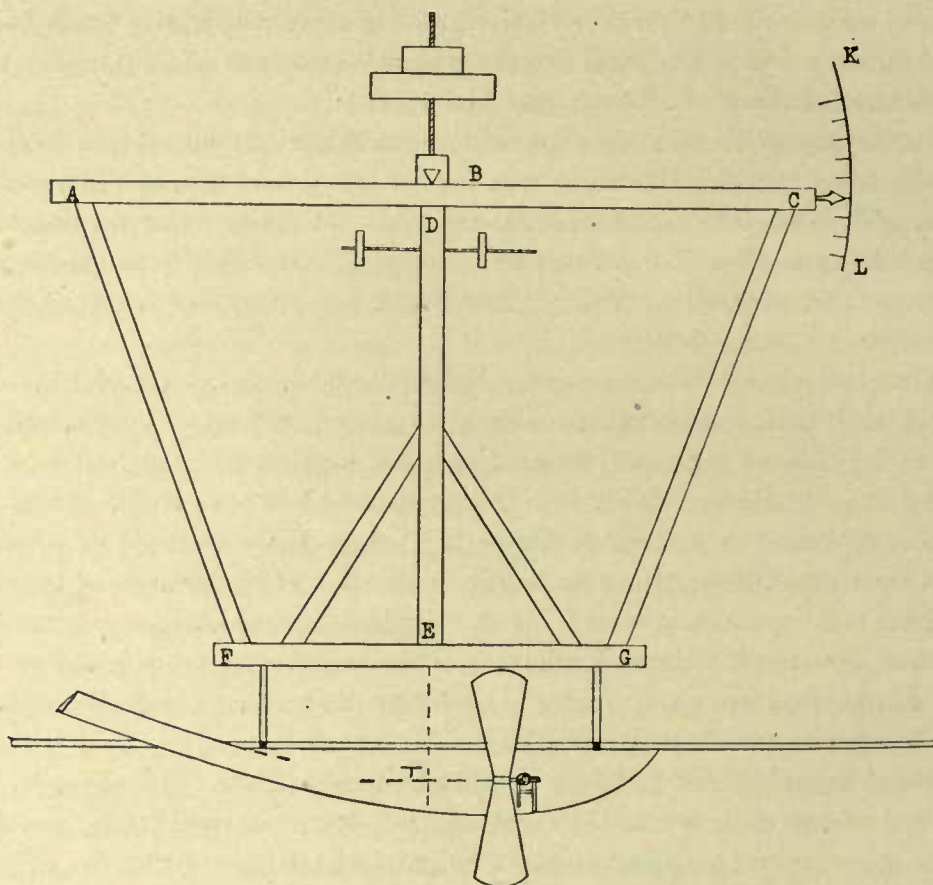
FIG. 10. Diagram of pendulum.
