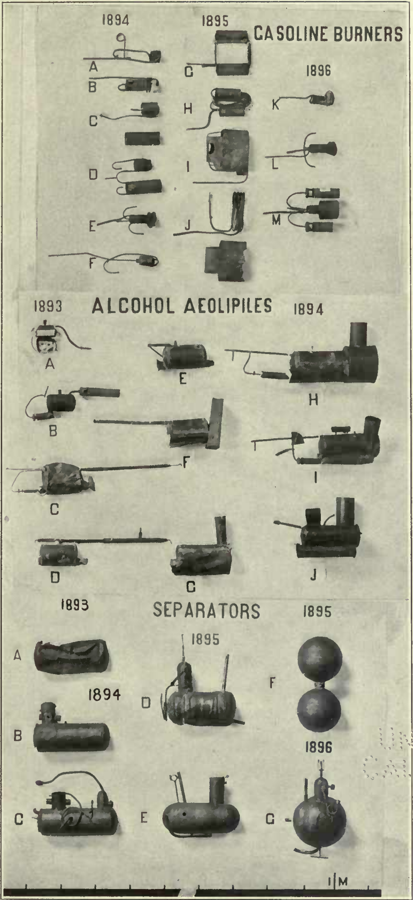
BURNERS, AEOLIPILES, AND SEPARATORS
