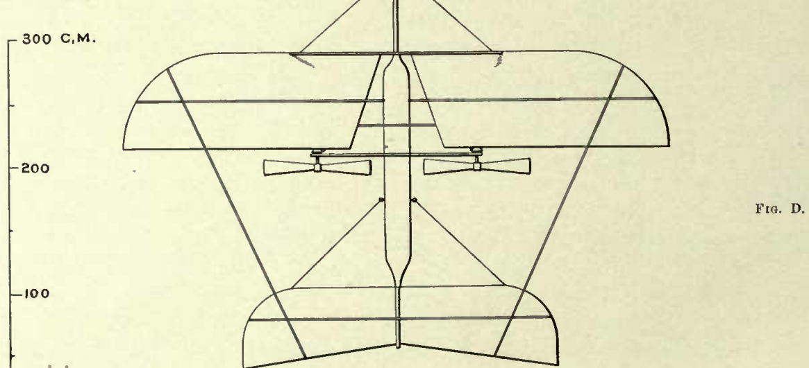
EARLY TYPES OF WINGS AND SYSTEMS OF GUYING
