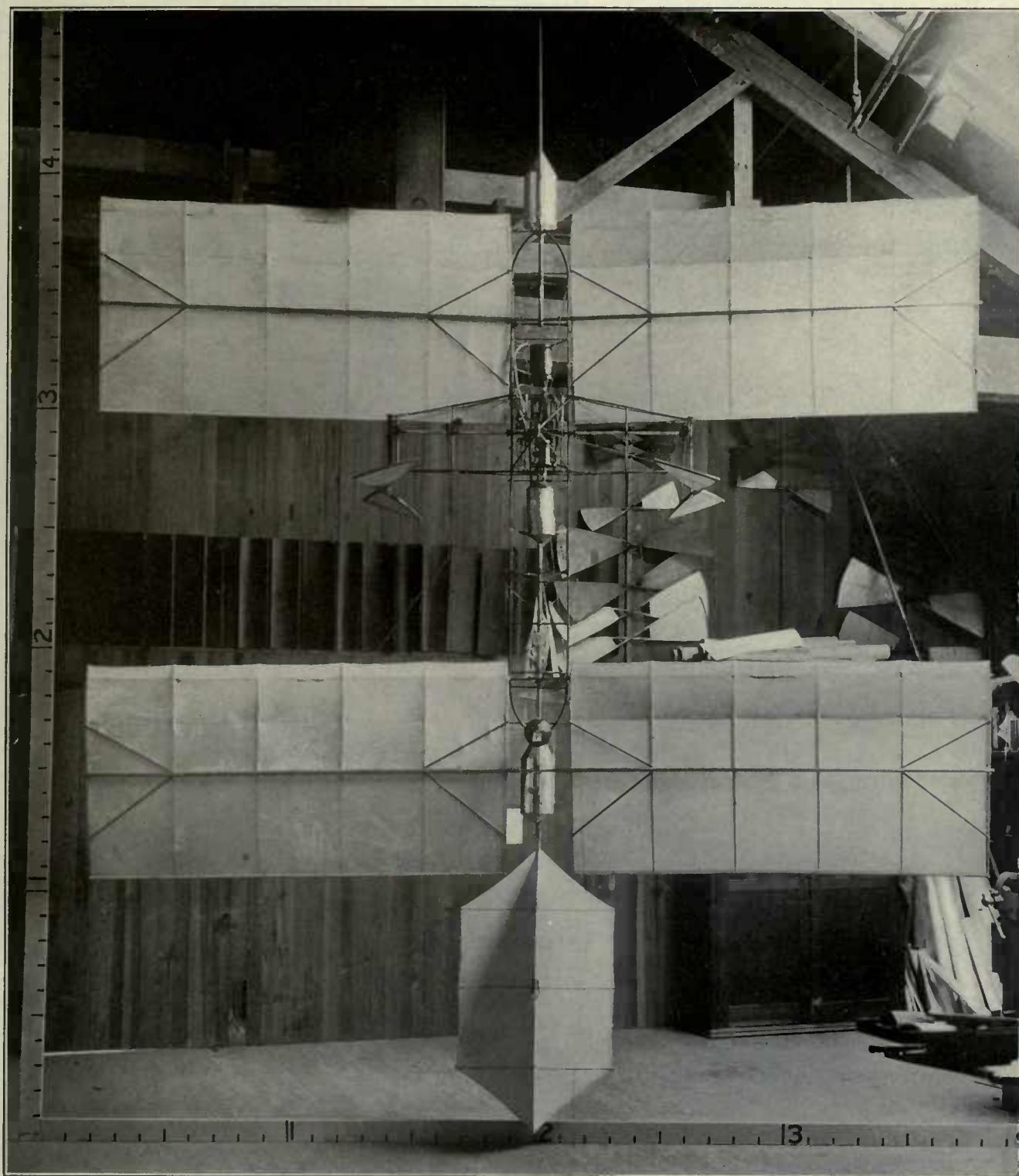
PLAN VIEW OF QUARTER-SIZE MODEL AERODROME
