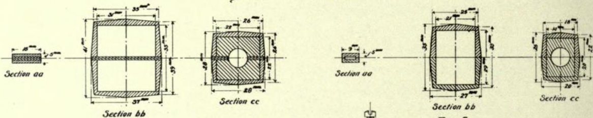
Fig. 9. Intermediate Cross Ribs.
