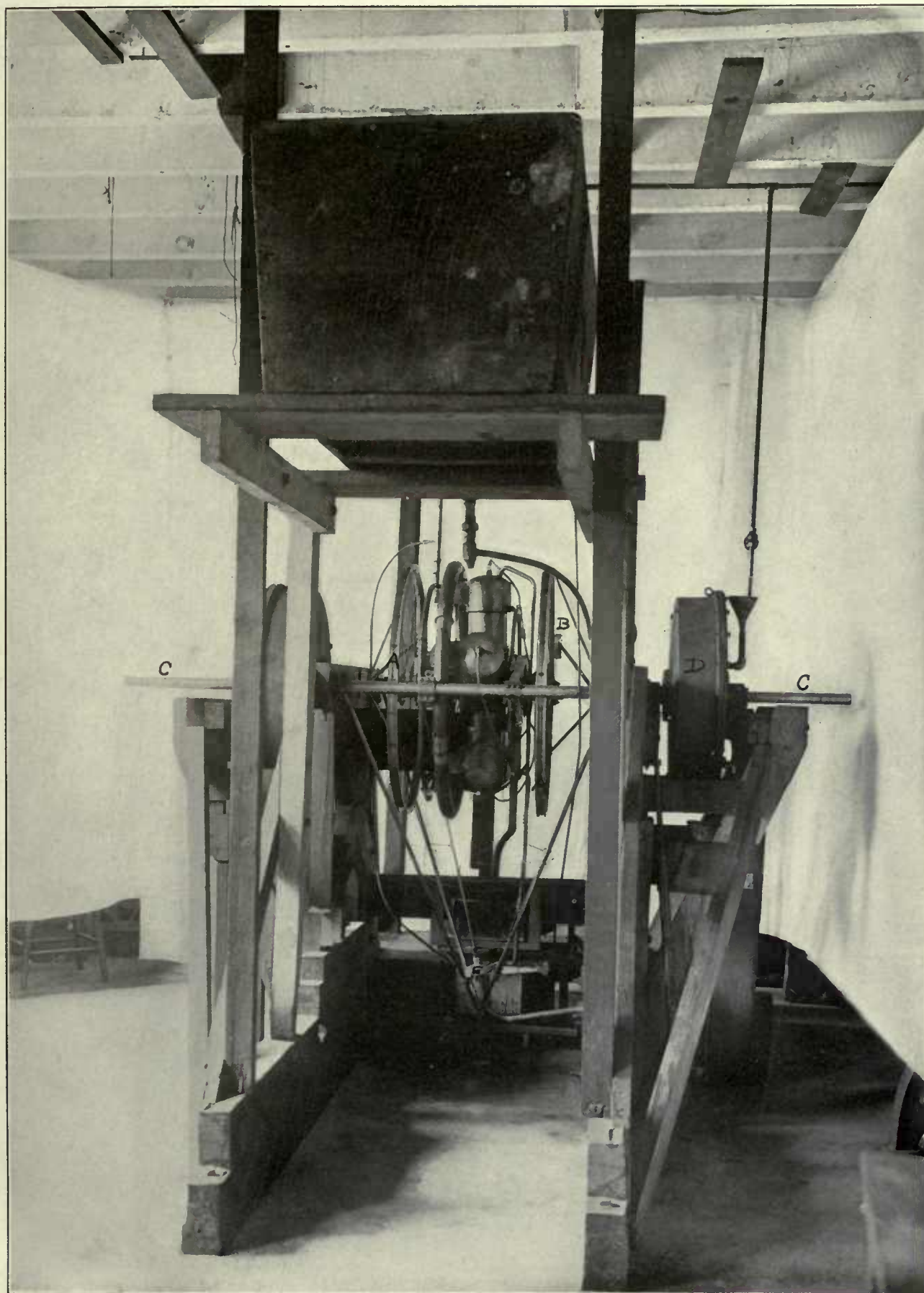
DYNAMOMETER TESTS OF LARGE ENGINE
