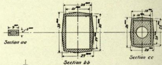
Fig. 9. Intermediate Cross Ribs.
