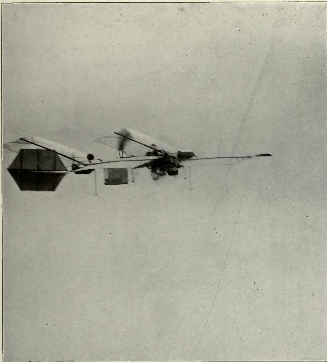
QUARTER-SIZE MODEL AERODROME IN FLIGHT, AUGUST 8, 1903
