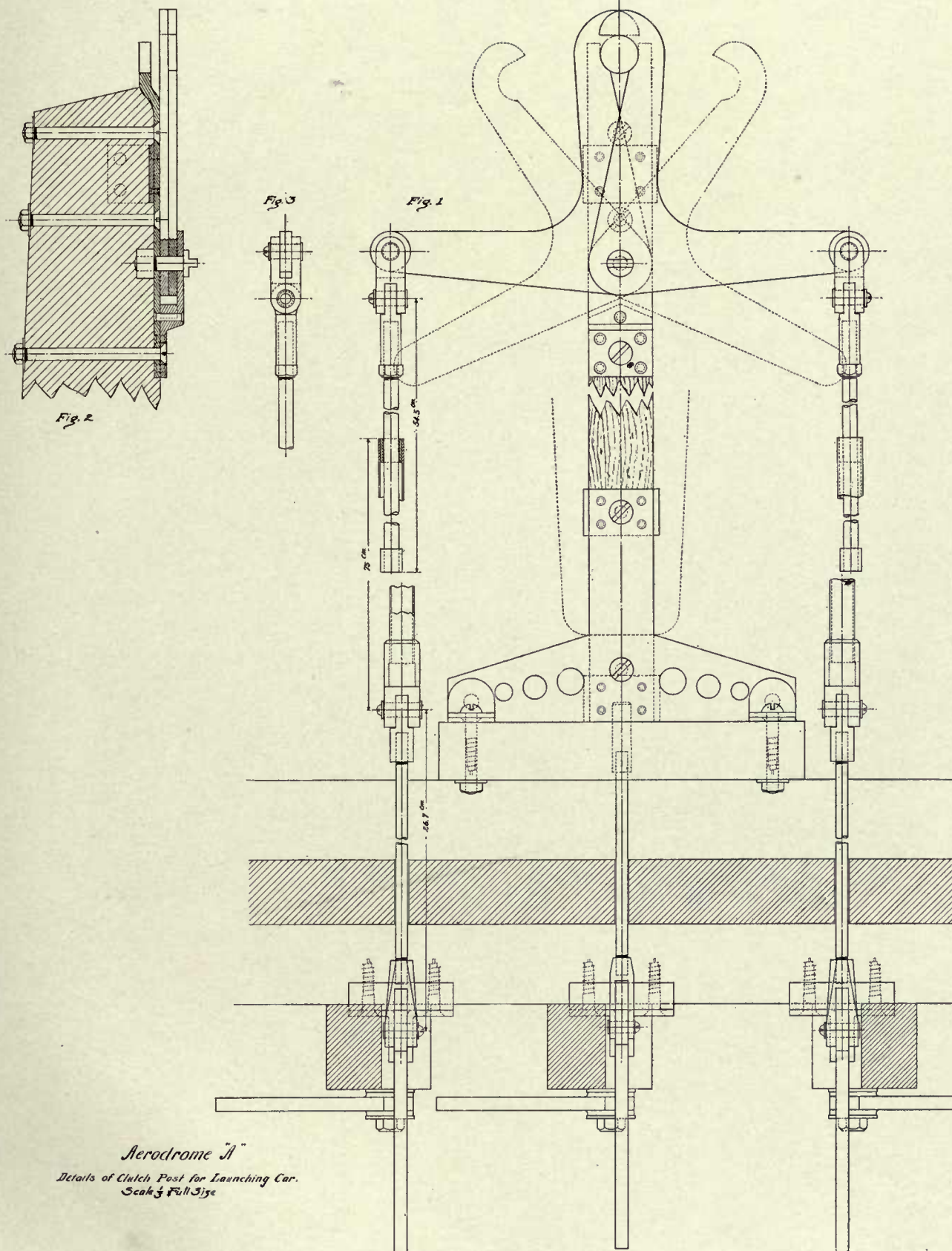
DETAILS OF CLUTCH POST FOR LAUNCHING-CAR
