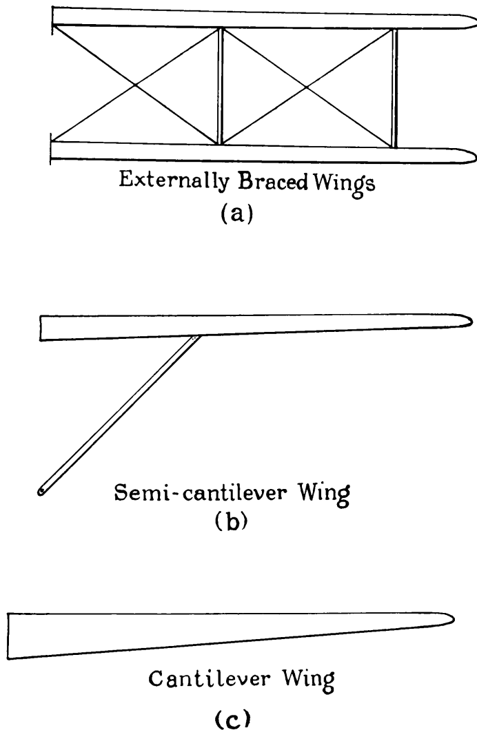
FIG. 113.—Three types of wings. (a) A good many struts and wires relieve the wing of much of the strain. (b) Has fewer struts and wires. (c) The wing itself bears all the strain.
