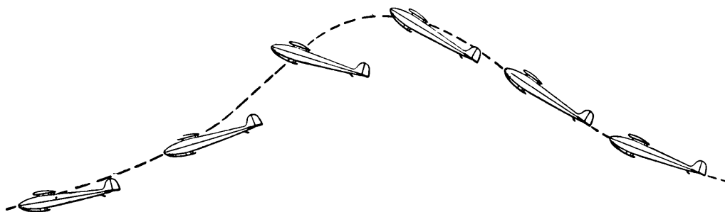
FIG. 100.—Movement of glider during stall. The dotted line shows path of plane going through stall.
