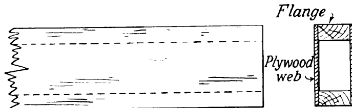
FIG. 120.—A box spar. This is a hollow box built of plywood. It is a uselessly expensive type of spar for fairly low-performance gliders.
