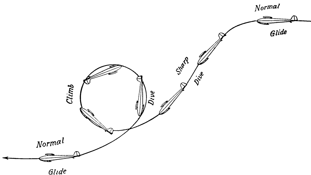
FIG. 102.—A loop. This diagram shows the glider's path of flight during one of the most hazardous of stunts.
