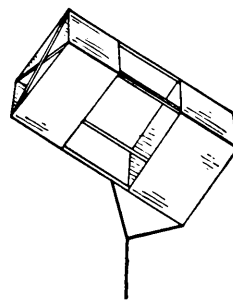
FIG. 35.—Position in which the kite flies. The harness is attached to the bottom of one of the corner sticks.
