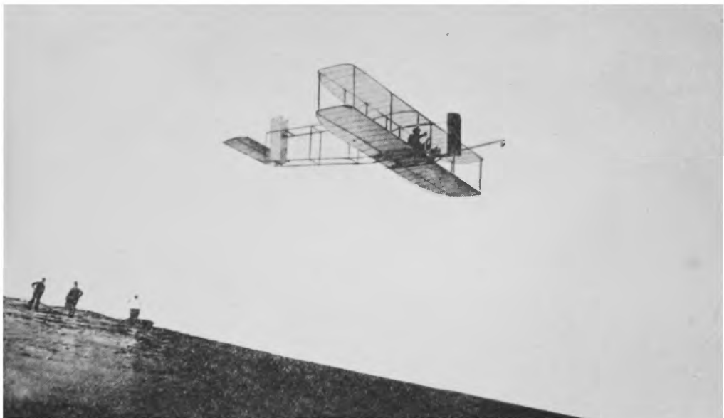
FIG. 16.—The Wright glider of 1911. This glider, in which a record was set, has a control system very similar to the one used at present.
