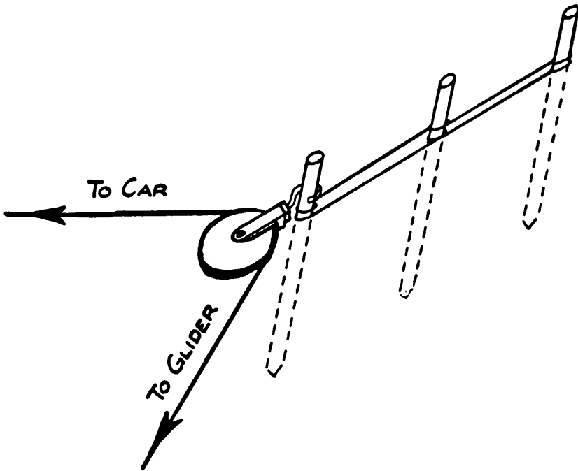
FIG. 29.—Pulley Fixture for Auto-Launching.
