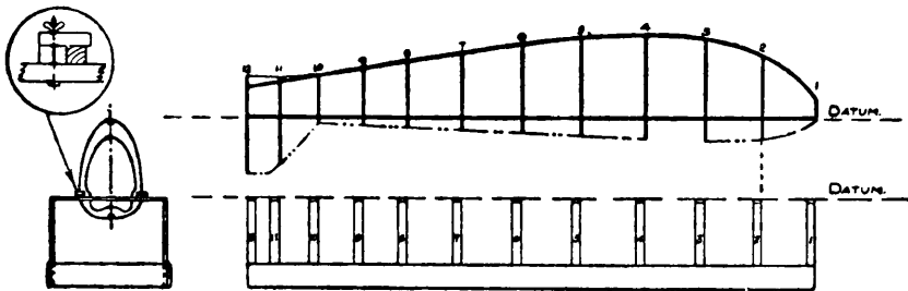
FIG. 36.—Fuselage Construction.
