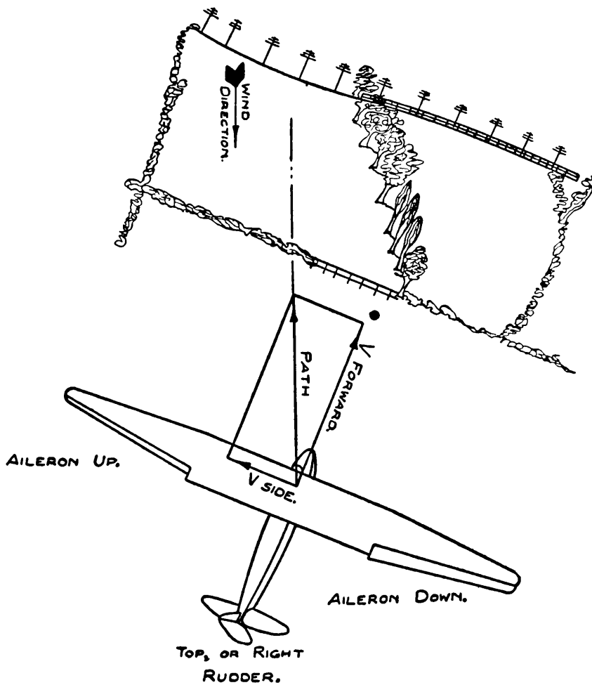
FIG. 27.—Landing Approach by Means of Sideslip.
