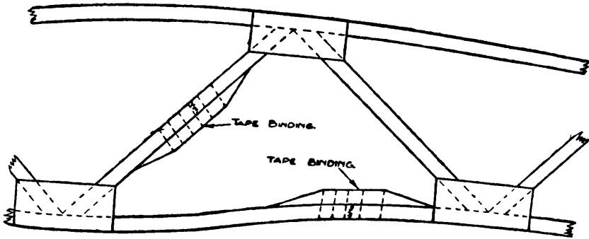
FIG. 41.—Repairs to Rib.
