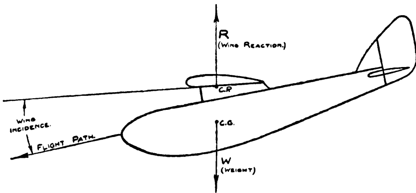
FIG. 7.—Forces on Glider in Normal Flight.
