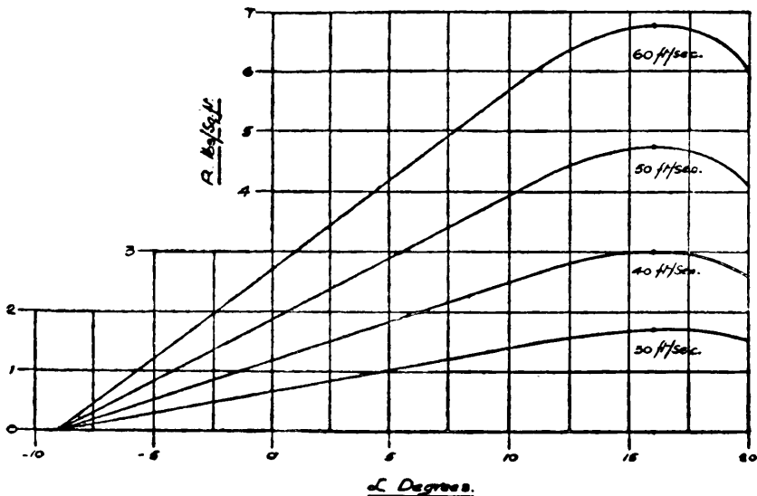
FIG. 4.—Air Reaction on Wing at Various Speeds.
