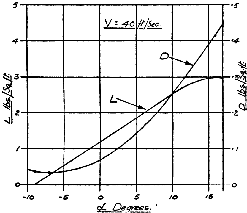
FIG. 5.—Lift and Drag Forces on Wing.
