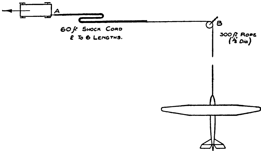
FIG. 28.—Auto-Launch.
