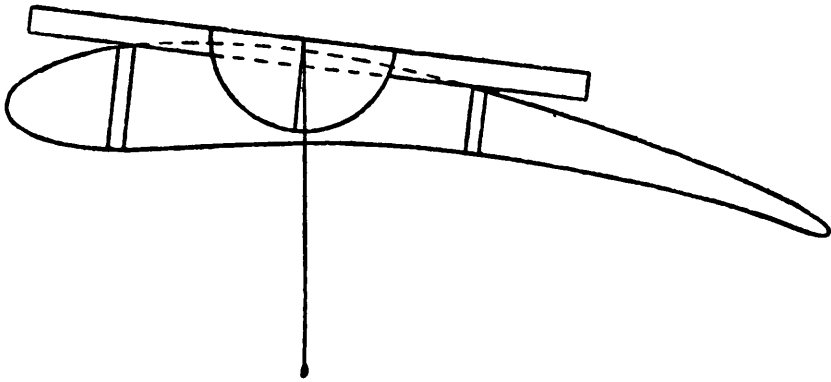
FIG. 15.—Incidence Board.
