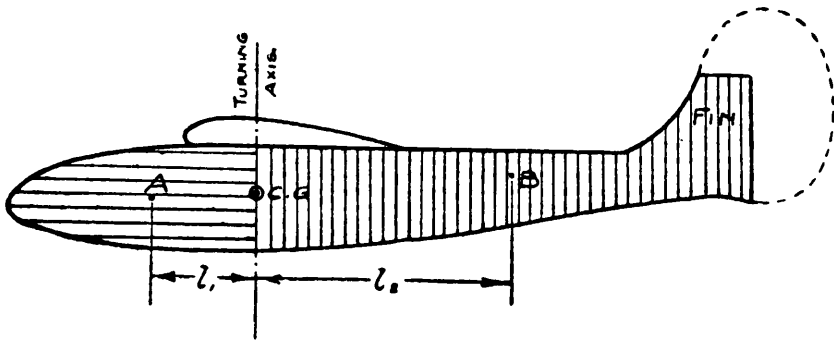
FIG. 12.—Directional Stability.
