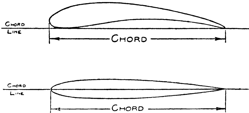
FIG. 3.—Aerofoil Sections.
