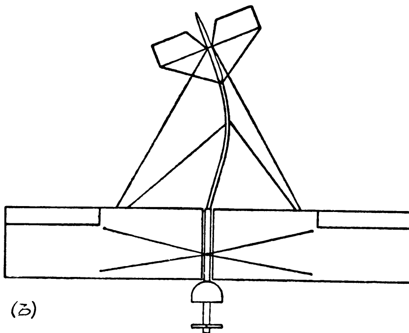
FIG. 16.—Rigging Faults.
