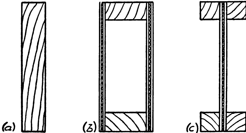
FIG. 30.—Spar Types.
