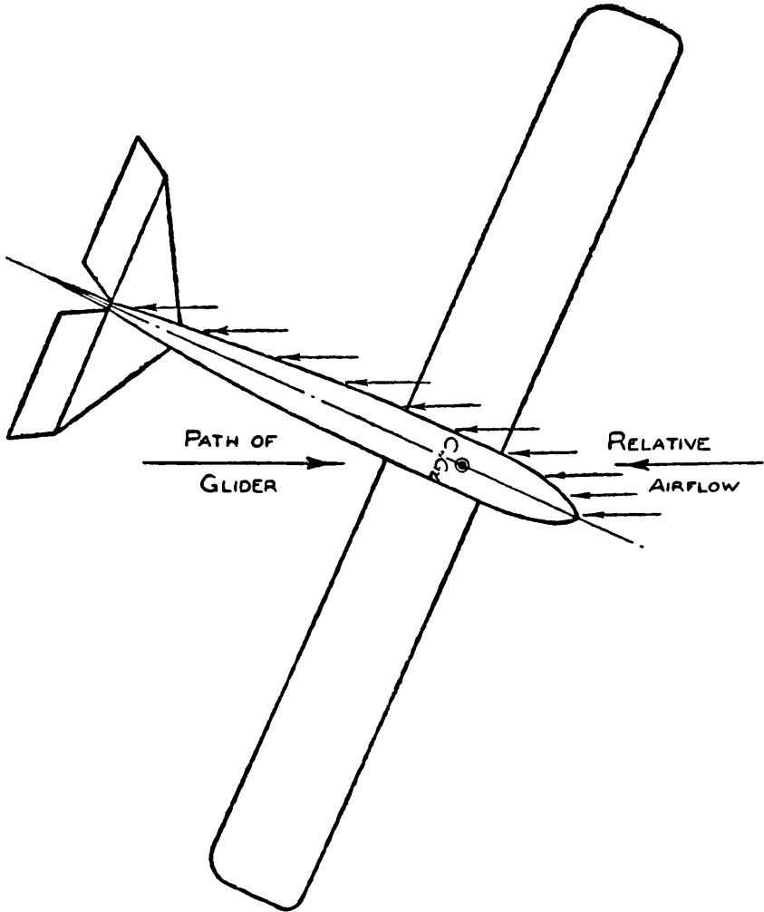
FIG. 11.—Directional or Weathercock Stability.
