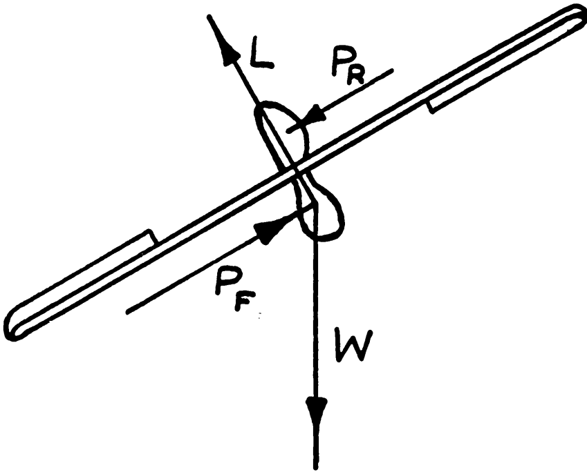
FIG. 24.—Forces Acting in a Sideslip.
