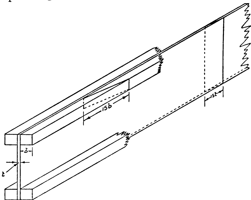
FIG. 31.—Splices in Spar.
