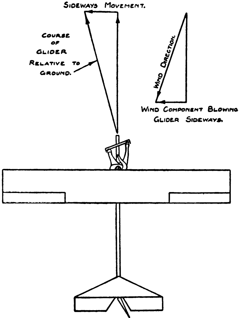
FIG. 19.—Correction of Drift.
