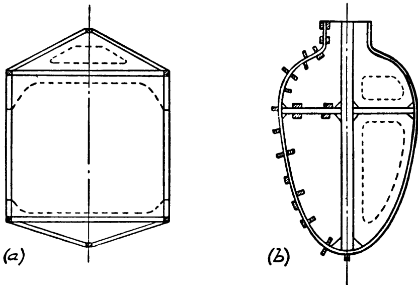
FIG. 35.—Construction of Fuselage Frames.
