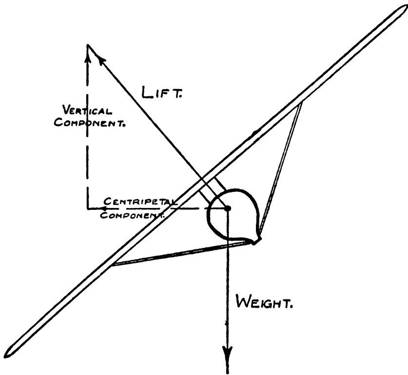
FIG. 13.—Forces in a Turn.
