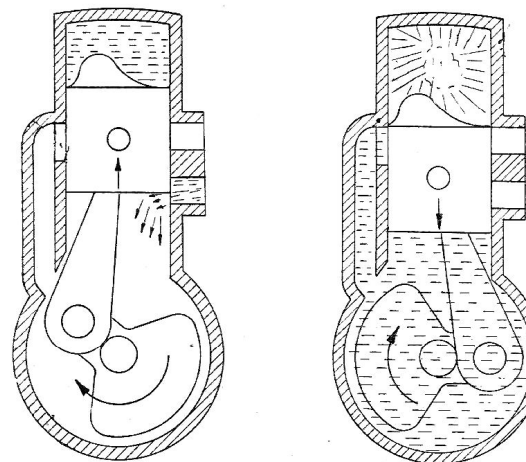
PISTON RISES SUCKS GAS INTO CRANKCASE COMPRESSES GAS IN CYLINDER
