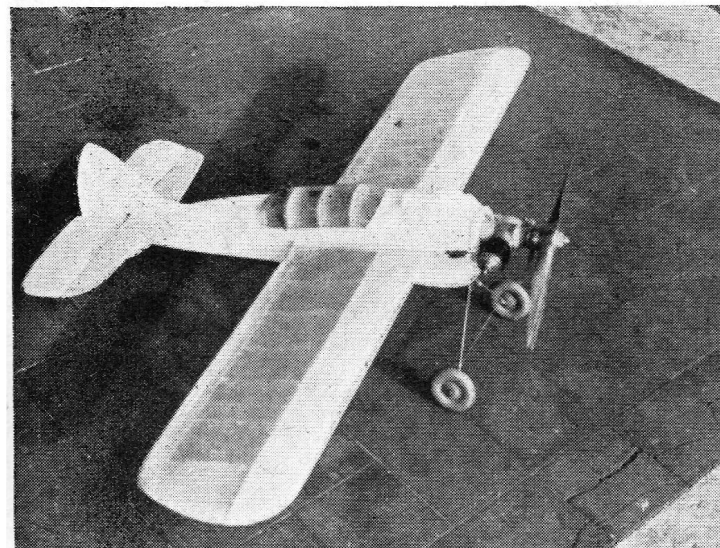
Fig. 30—This control line model drops its undercarriage after take-off. The propeller is so arranged that when the engine stops the propeller will be horizontal and ready for a "belly landing." Less drag and better stunting is the result.
