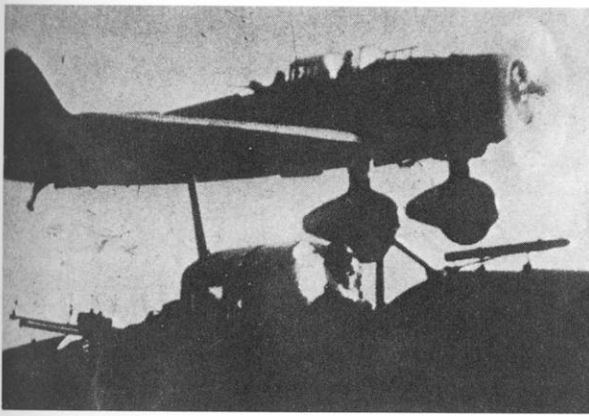
A pair of D3A1s in close formation. Details of the external bombsight and drum-fed Type 92 flexible rear-firing machine gun are clearly visible on the aircraft in the foreground.
