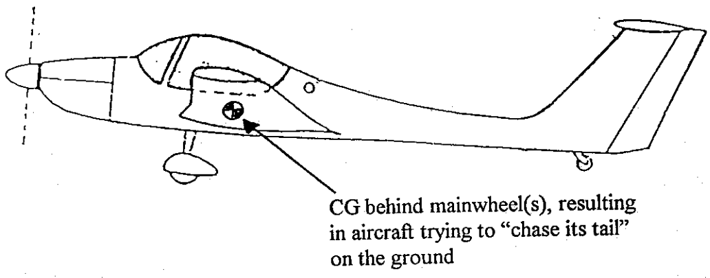
Grob G109B, showing reason for directional instability
