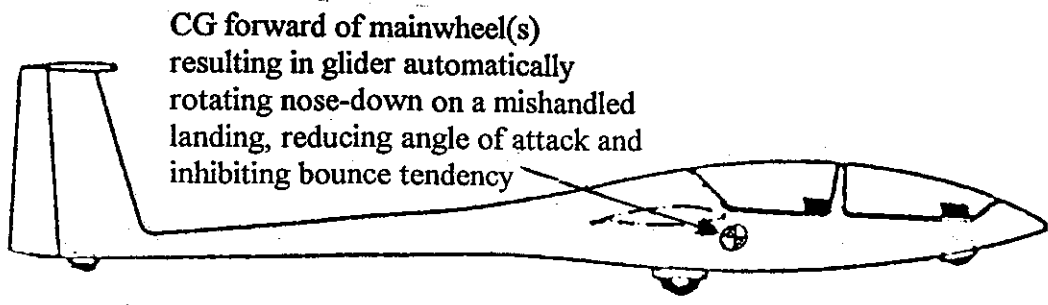
Glaser-Dirks DG500M, showing anti-bounce characteristic
