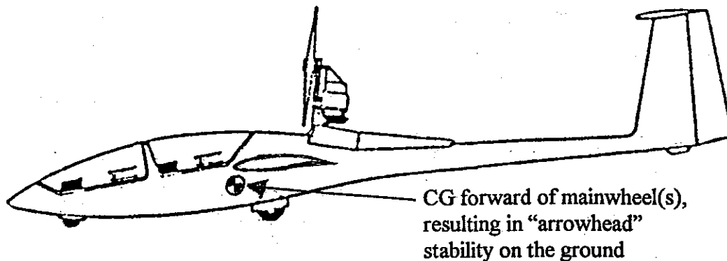
Glaser-Dirks DG500M, showing reason for directional stability
