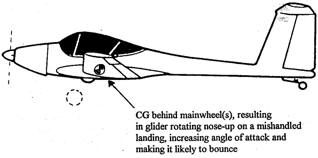
Brasov IS28M2, showing why taildraggers tend to bounce
