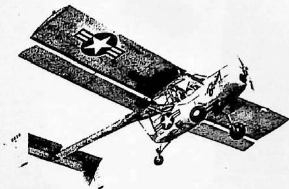
The unique Boeing Model 451, the XL-15 Scout, in flight. Note separate 'flaperons'. (Boeing Photo 2B-3427)
