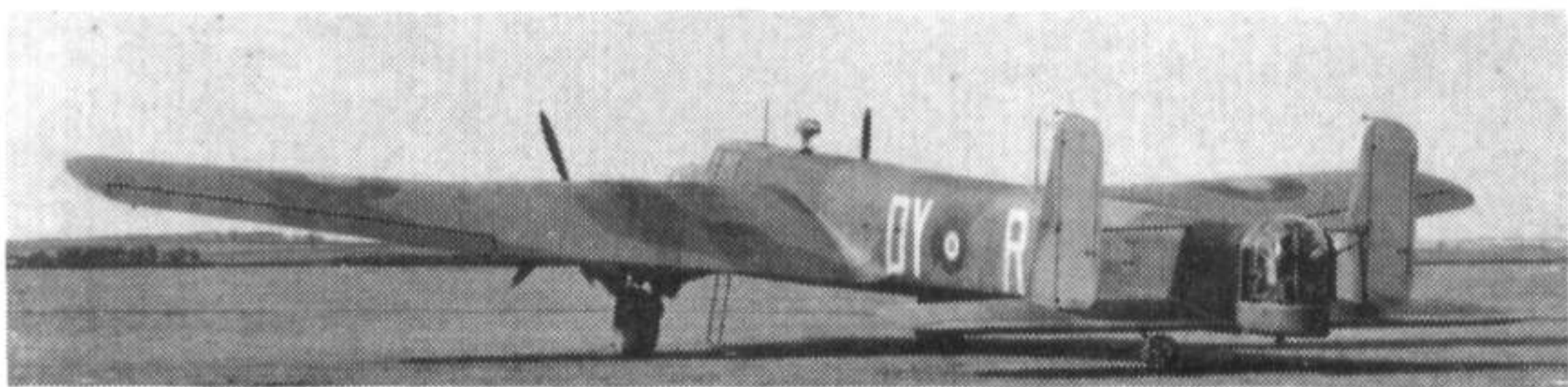
Mk. V N1380 "DY-R" of No. 102 Squadron, subject of the 5-view drawing on pp. 8 and 9. (Photo: "The Aeroplane")
