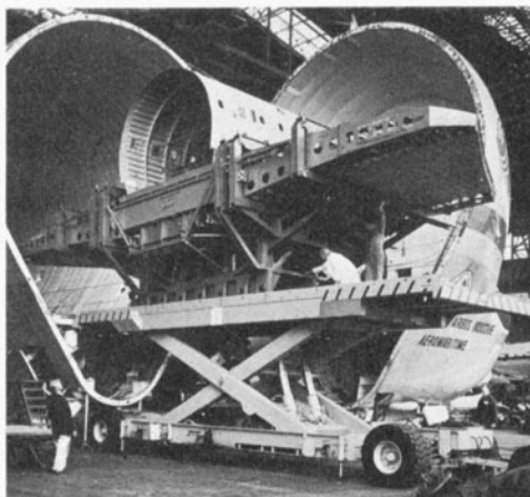
Concorde centre fuselage and wing section (Component 15) being unloaded from the Aéro maritime 'Super Guppy' freighter at Filton.
