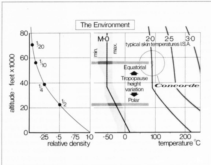
The physical characteristics of the International Standard Atmosphere—notably the variation of relative density, Mach Number and temperature with altitude, and (right) the added effect of kinetic heating at SST Mach Numbers. Overlaying this picture in practice are further variations due to climatic effects.
