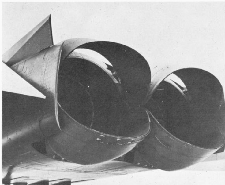
Close-up of a pair of the TRA (Thrust Reverser Att) variable-area engine exhaust nozzle and thrust reverser/silencer 'clamshell bucket' units.
