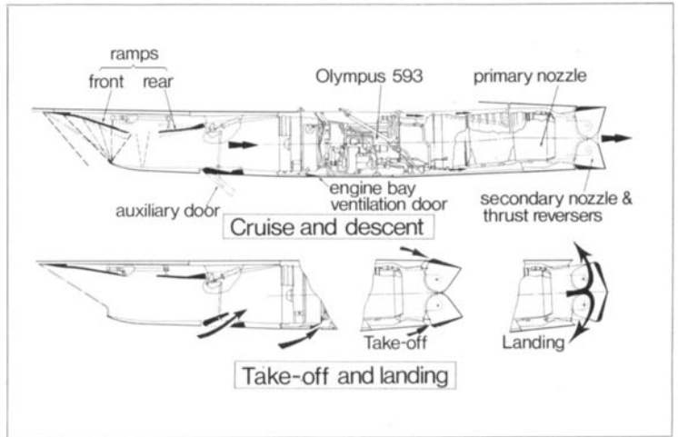
Sequence of operation of variable geometry powerplant air intake and exhaust systems.
