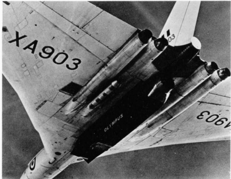
Underside view of the Olympus-Vulcan flying engine test bed aircraft incorporating a full-scale facsimile of one of Concorde's power-plant units (but with the earlier-type exhaust system)
