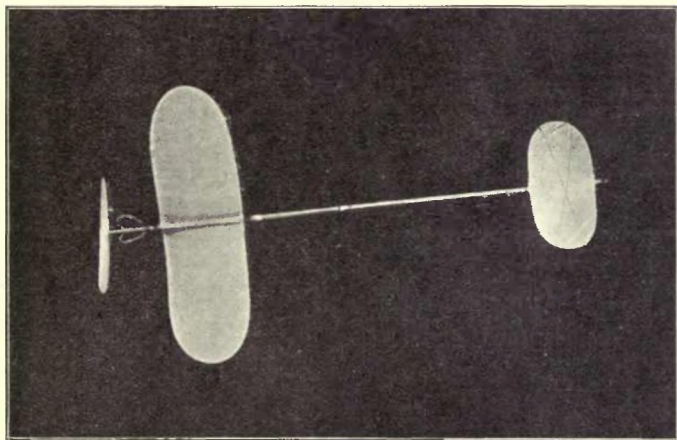
FIG. 58.—MODEL DESIGNED AND CONSTRUCTED BY THE AUTHOR FOR "GREATEST HEIGHT."
