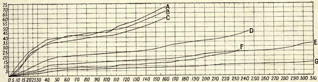
FIG. 16.—TORQUE GRAPHS OF RUBBER MOTORS.
