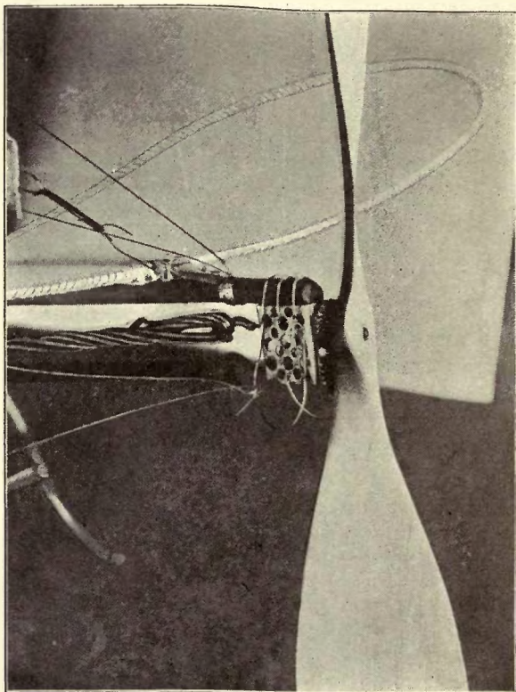
FIG. 17.—GEARED RUBBER MOTOR.
