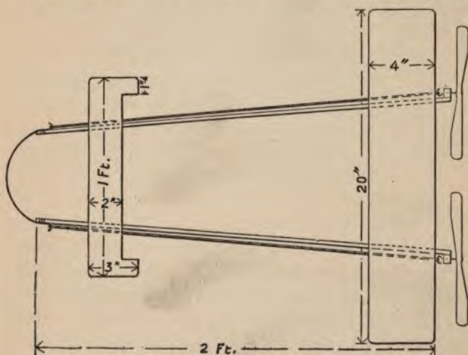
AN EFFICIENT THREE-OUNCE MODEL.
