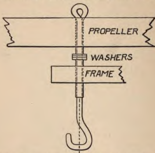
SHOWING CONSTRUCTION AND MOUNTING OF PROPELLER AND AXLE.
