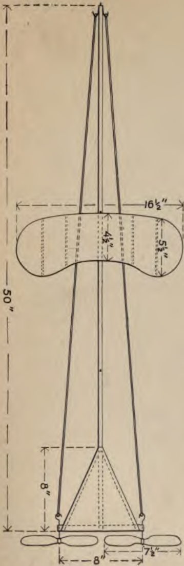
Working drawing of the Fleming Williams model
