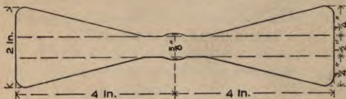
LANGELEY PROPELLER BLANK.
