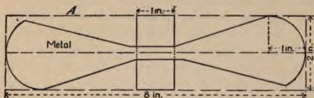
DESIGN OF METAL PROPELLER.
