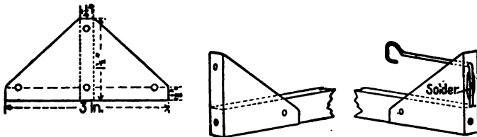
A METAL MOTOR ANCHORAGE.
