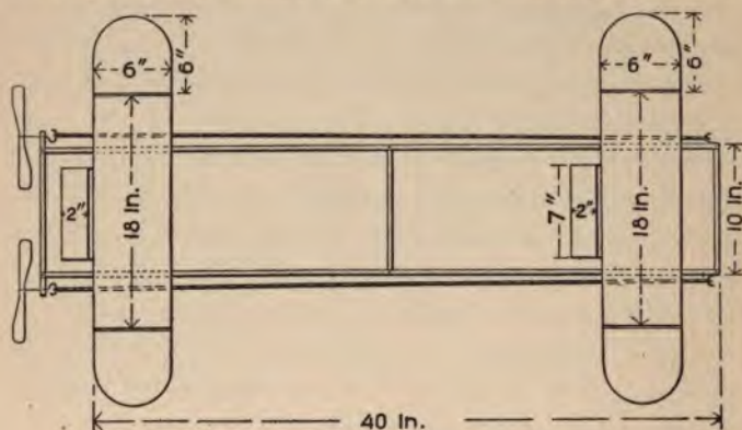
A MODEL WITH ADJUSTABLE STABILIZER.
