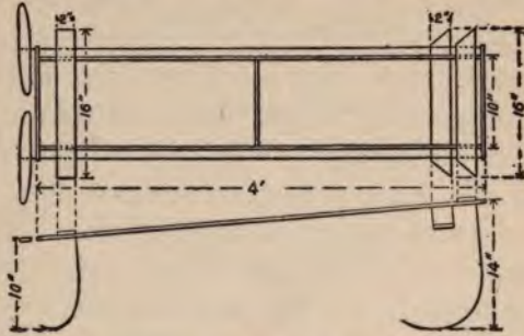
MODEL WITH MINIMUM PLANE SURFACE.
