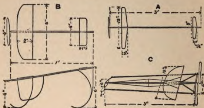
A—THE FAMOUS "ONE OUNCER." B—A SMALL EXPERIMENTAL MODEL. C—A MODIFIED BURGESS WEBB MODEL.
