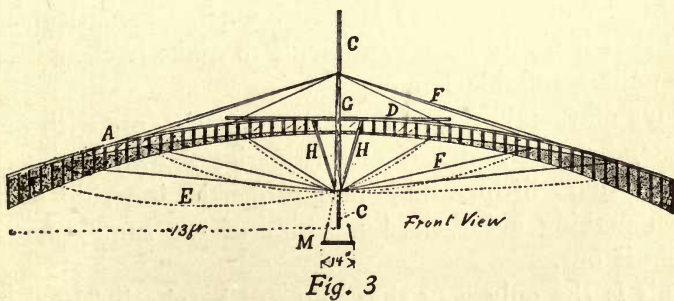
DETAILS OF MONTGOMERY GLIDER CONSTRUCTION
