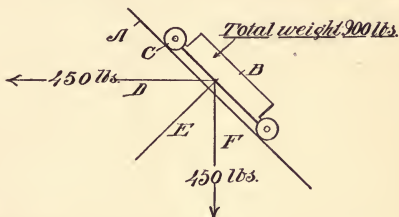
Fig. 60. Horizontal and vertical pull.
