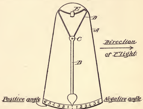
Fig. 66. Angle Indicator.
