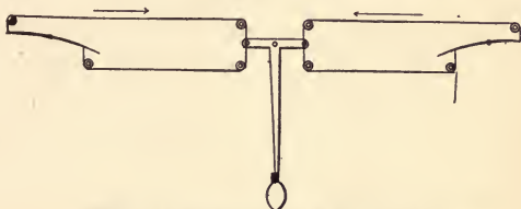
Fig. 68. Pendulum Stabilizers.
