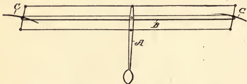
Fig. 67 Simple Pendulum Stabilizer
