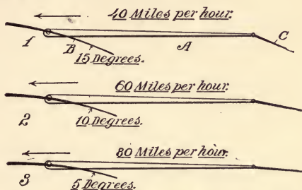
Fig 13. Planes on Non-Changing Body.
