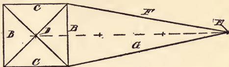
Fig. 49. Rule for Spacing Planes.
