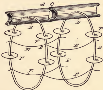
Fig. 38. Ribs of Dragon Kite.
