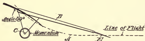
Fig. 20. Action when Propeller ceases to pull.
