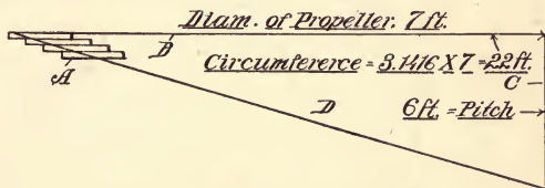
Fig. 77. Laying out the Pitch.
