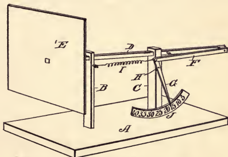
Fig. 62. Air Pressure Indicator.
