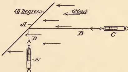
Fig. 6. Measuring Lift and Drift.
