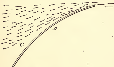
Fig. 25. Air lines above a convex Plane.
