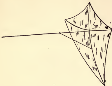
Fig. 34. The Malay Kite.
