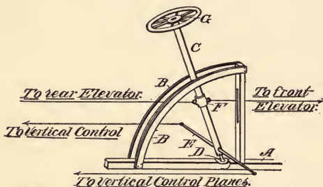
Fig 69. Steering and Control Wheel.
