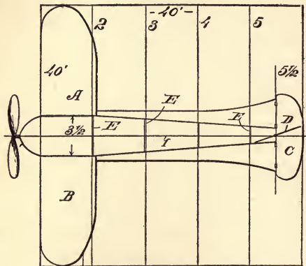
Fig. 58. Plan of Monoplane.
