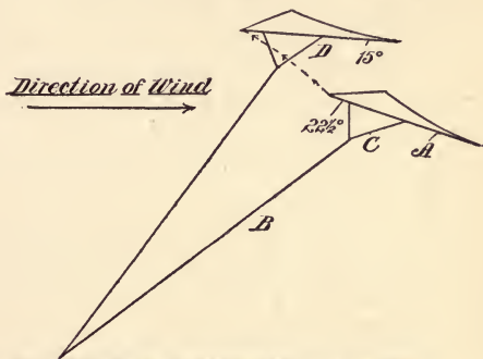
Fig. 48. Action of wind forces on Kite.
