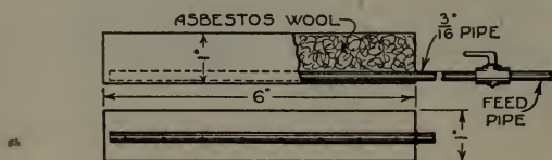
Fig. 182—The alcohol burner used to fire the boiler
