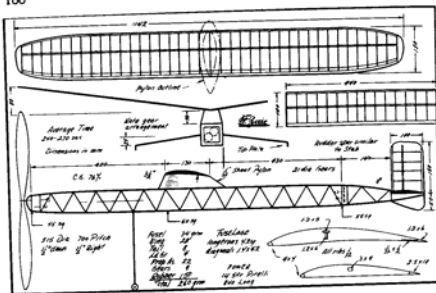
Figure 21. Another top Wakefield of its day, by Gunter Maibaum of Germany. (F. Zeig drg.)
