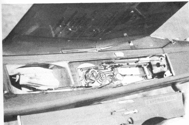
Complex Seelig timer connections are a pre-requisite for flappers. Left is bladder tank housing, centre the timer and right the leads to tail and flap controls.
