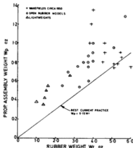
FIGURE 13 DEPENDENCE OF PROP ASSEMBLY WEIGHT ON RUBBER WEIGHT
