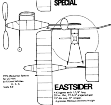
Two more Whitten designs, appropriately named as their home is in the heart of Manhattan Island. Eastsider placed 5th in the Nats event to gain Jr/Sr First prize.
