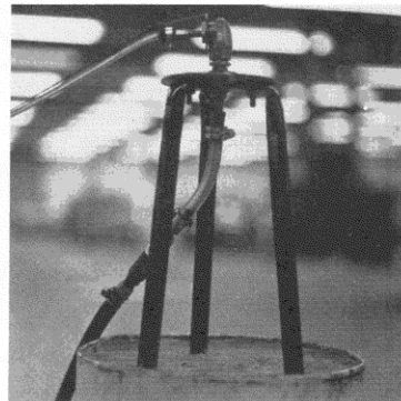
The complete pylon, with its three legs firm in the concrete set in top of a 5 gallon oil drum.
