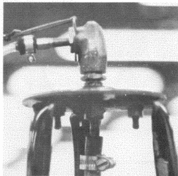
Vital head on the pylon made from a Tecalet grease elbow, mounted securely and rotating freely.
