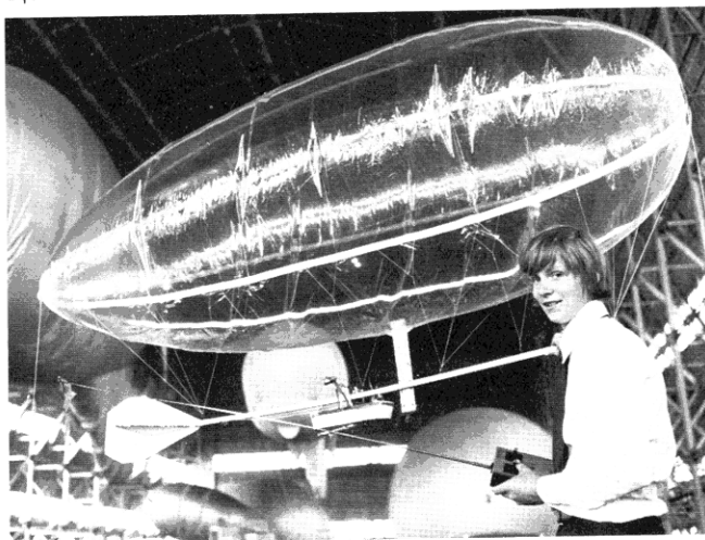
Richard Barnes-Gorell controls the "Bournemouth 4" in the airship shed at R.A.E., Cardington. It takes 43.5 cu. ft. of Helium to fill the Meline envelope. Propellers swivel for thrust vector control. C.O.I. photo.
