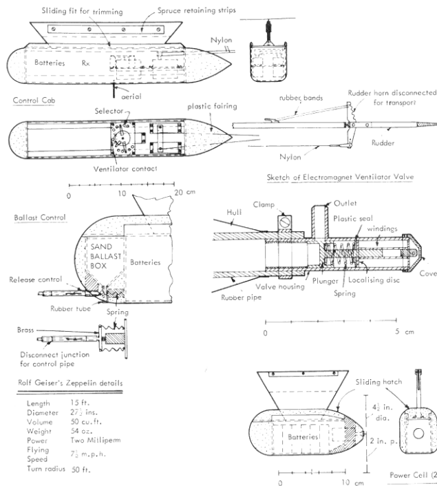
Details of a radio controlled "Zeppelin" by Rolf Geiser which made many demo's in Switzerland and Germany during 1976—courtesy "Flug-Technik". Note the electro-magnetic control valve.
