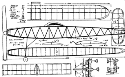
Figure 7. Aarne Eklis's (Finland) Wakefield won the World Championship in 1949 and 1950. the first winner to use twin motors and return gears. (F. Zaic dig.)
