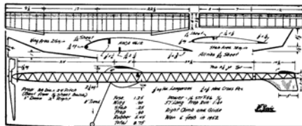
Figure 8. Typical of the very long Wakefields to emerge in 1952. This is designed by George Perryman (U.S.A.). (F. Zaic dig.)
