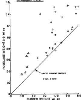
FIGURE 12 DEPENDENCE OF FUSELAGE WEIGHT ON RUBBER WEIGHT
