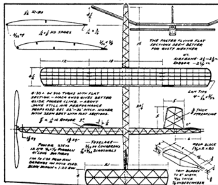
Figure 18. Another typical but smaller unrestricted model design, Goblin Able by N. P. Elliott. (F. Zaic dir.)
