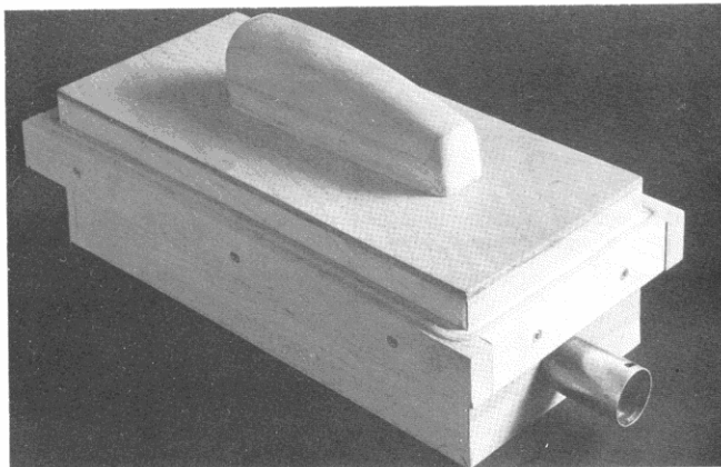
Vacuum table with plug in position. Note built-up plug. Note holes in table top, surgical tube seal, masking tape seal around bottom edge and general construction. Photo by Thorney Lieberman.
