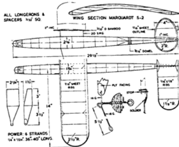
Figure 17. Thermal Bug by Brian Lewis, together with Suga Dups, recorded the highest duration potential of all the models for which data is known.
