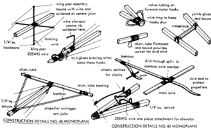
Clark Mono- planes Flight February 1912
