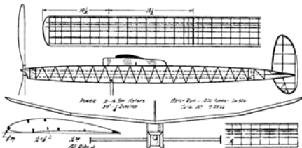
Figure 9. Winner in 1953. W. Forster (U.S.A.) used twin motors and appropriately named his model "Power/Weight". (F. Zeigler)
