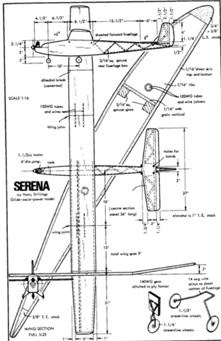
DESIGNER'S G/A SKETCH
