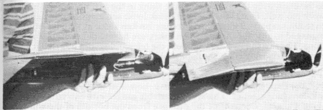
Flap up for climb, down for glide on Meta-Nemesis.
