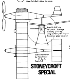
Hank Nixon's Stonycroft Special was widely publicized, aimed at the novice modeller.
