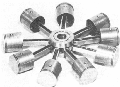
Pistons have two rings, and a cutaway in the skirt to give clearance for the piston in the next cylinder.
