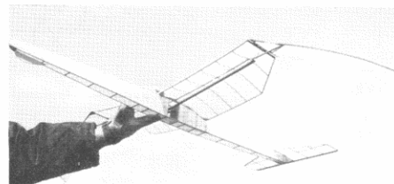
Top: Alex Imrie with the "Schwingenflugmodell" flapping tips raised, and at right, on the full downbeat. Close-up of the very simple connecting rod and crank mechanism, below, also emphasises the birdlike airfoil on the fixed wing.
