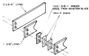
FIG. 4 SLOTTING FIXTURE. \frac{1}{8} "-Ø OIL-HARDENING TOOL STEEL UNLESS OTHERWISE NOTED
