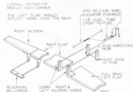
Linkage for a typical flap/hook/aileron system (in addition of course, to elevator and throttle).
