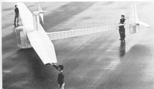
Covered with "gan hishi" Japanese paper, the newly built Stork in pristine condition.
