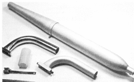
HP tuned pipe silencer with alternative steel and alloy elbows, PVC connection and clamps.
