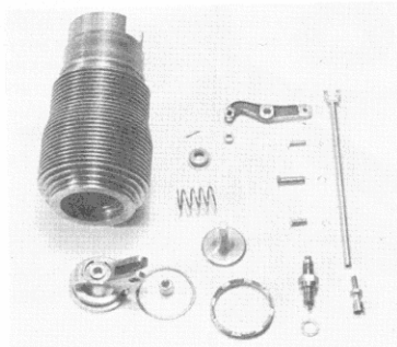
The valve gear. Spring is wound from piano wire, pushrods are actually Hypodermic needles! Pins are silver steel and machined from the solid.
