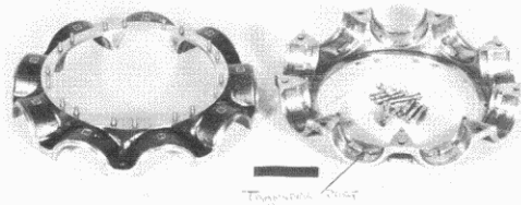
Transfer ports are cut into halves of the split crankcase. Black mark is one inch (25 mm.) long.
