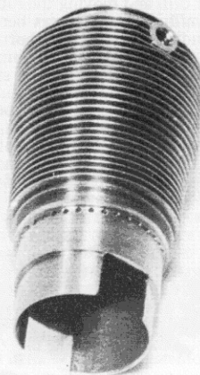
The one-piece cylinder barrel and head, note plug socket, transfer ports and cylinder retaining ring just above, which is clamped by crankcase.
