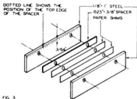
FIG. 3 SLIDE HOLDING FIXTURE. ALL PIECES 3\frac{3}{4} " LONG ALL HOLES \frac{1}{8} " Ø BOLT TOGETHER WITH \frac{1}{4} "-20 SCREWS
