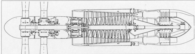
BMW 109-028. 6,700 hp shaft output turboprop version of the BMW 109-018 jet engine. Driving four-blade contra-rotating propellers and delivering 1,200 kg (2,645 lb) additional thrust, the BMW 109-028 turboprop was to have powered the BMW High-Speed Bomber Projects I and II.
