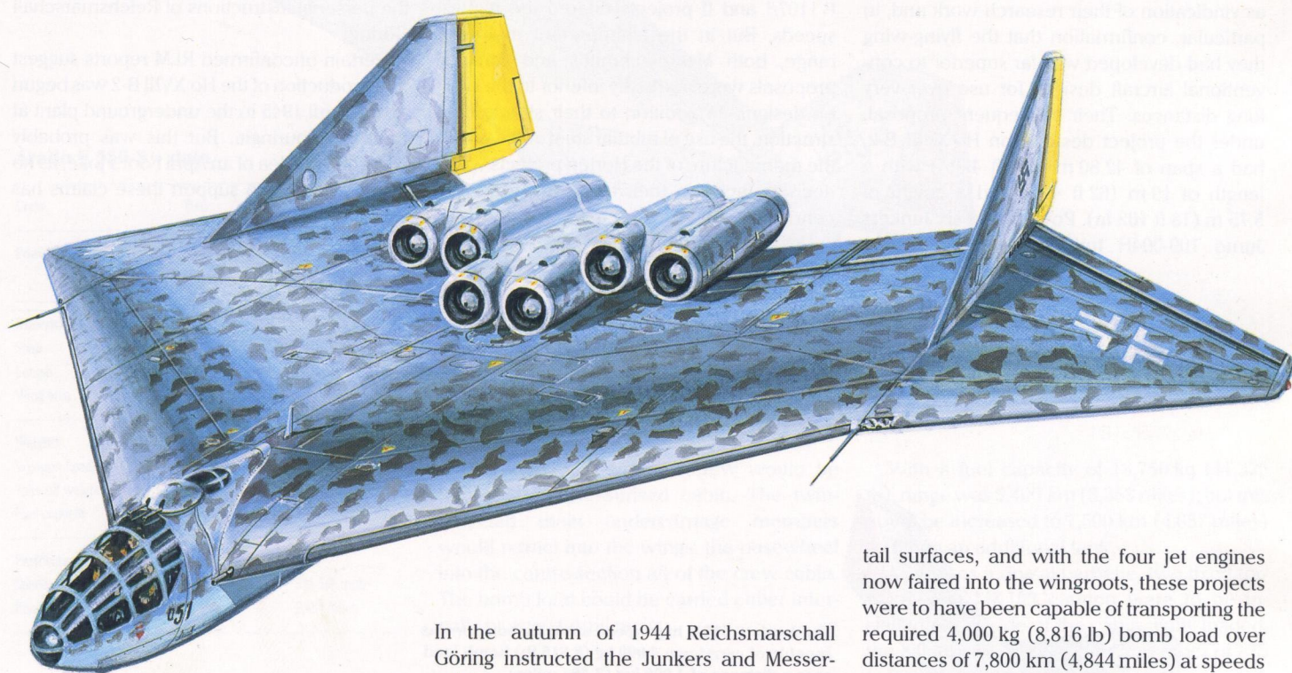
The Arado E 555-1 long-distance flying-wing bomber, the first design in the E 555 development series.
