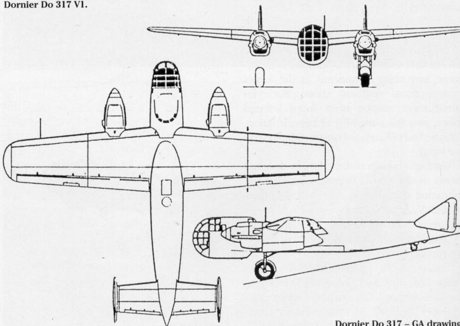
Dornier Do 317 – GA drawing.
