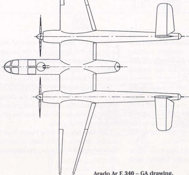
Arado Ar E 340 – GA drawing.
