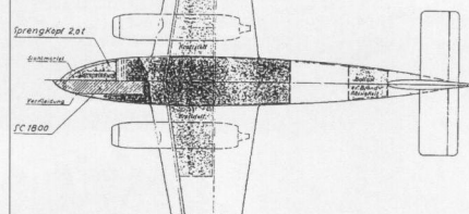
GA drawing of the Arado E 377 powered by two BMW 109-003 turbojets.
