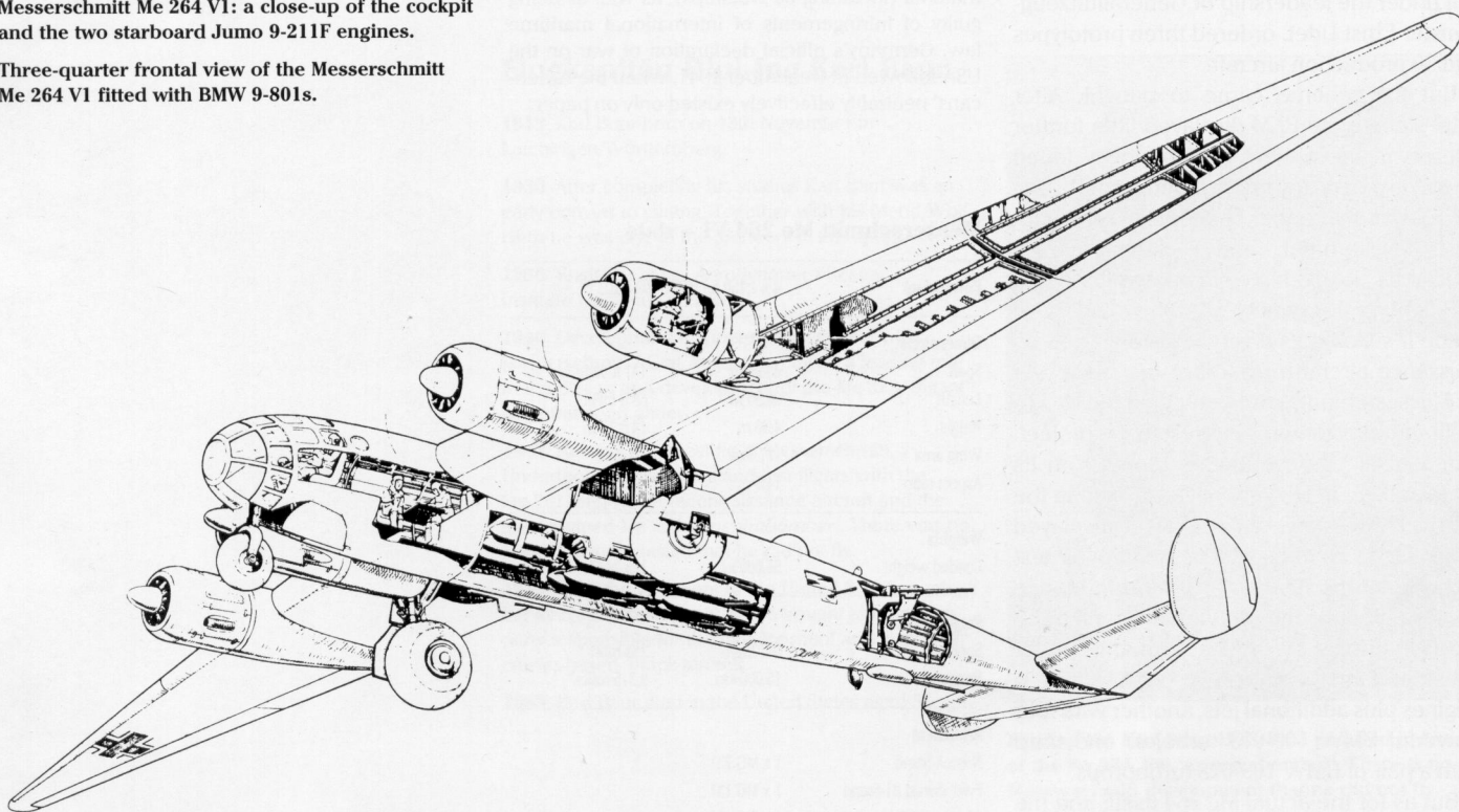
Partial cutaway of the Messerschmitt Me 264 in flight.
