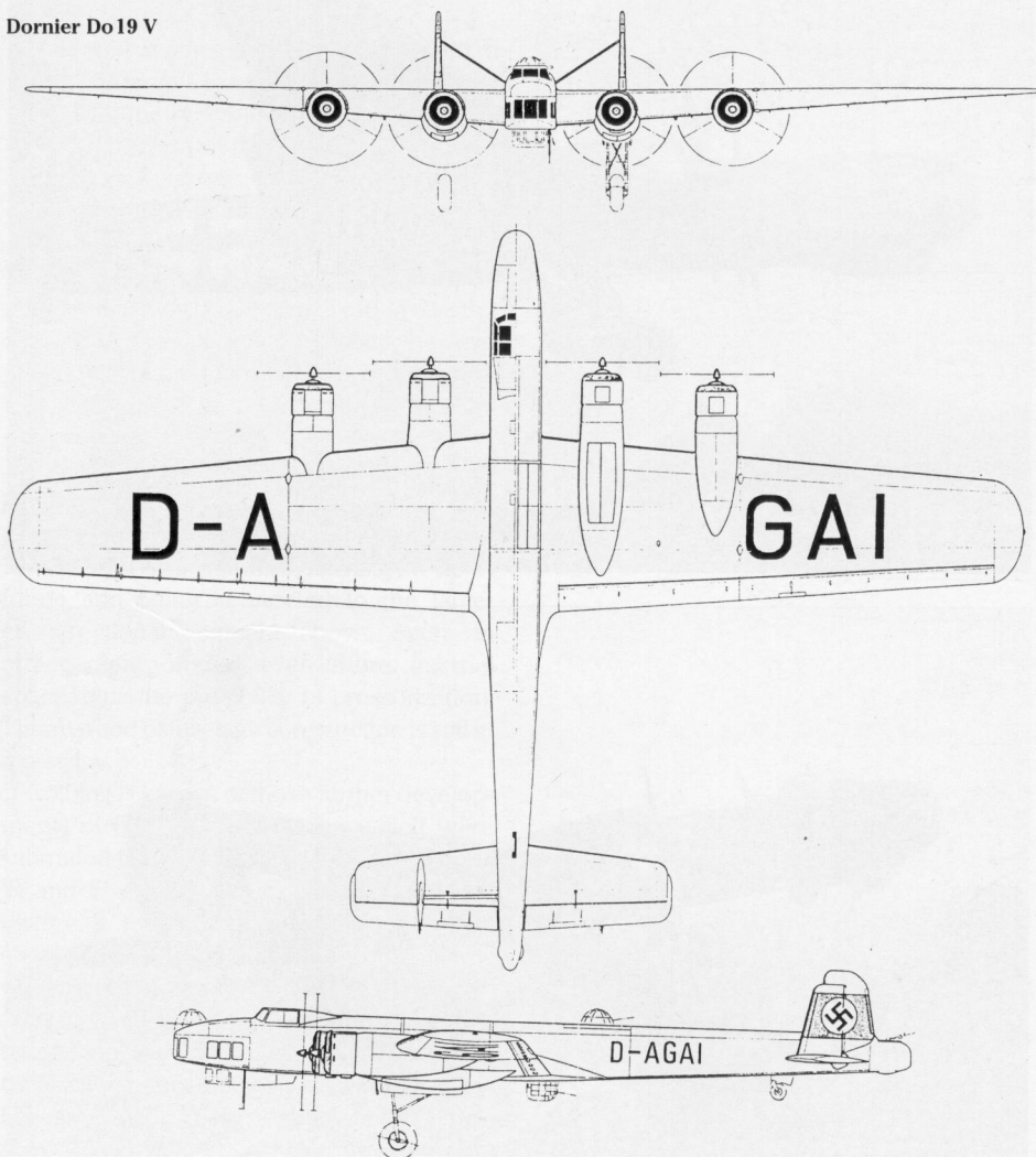
Dornier Do19 V
