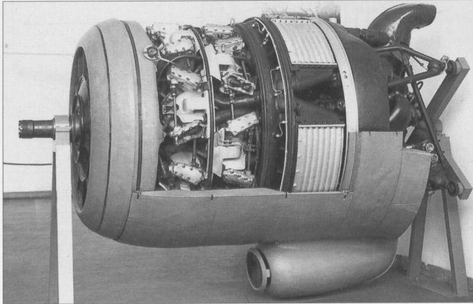
Top and above: BMW 801 TJ. 2,000 hp 14-cylinder twin-row high-altitude radial engine with exhaust gas turbocharger and charge cooling.
