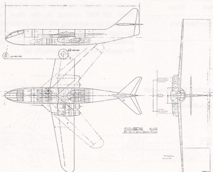
Messerschmitt P 1101/103 - GA drawing.
