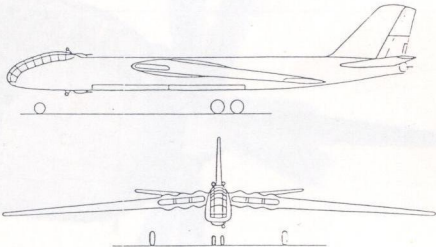
GA drawing of the Junkers EF 132.
