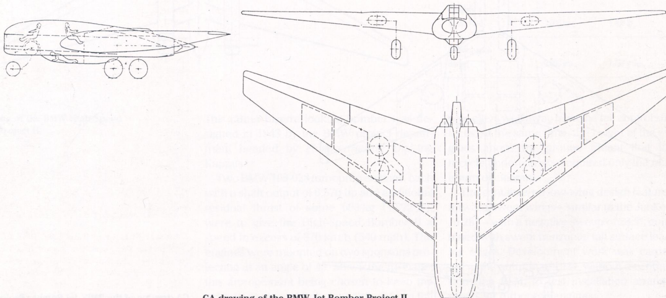
GA drawing of the BMW Jet Bomber Project II.
