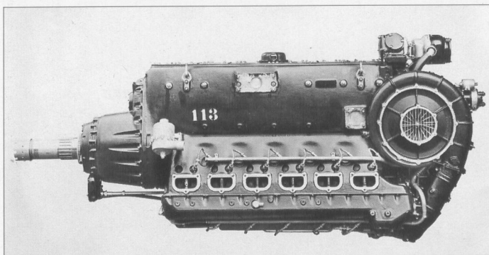
Daimler-Benz DB 603 ASM. 2,250 hp 12-cylinder injection engine, with additional MW-50 boost, which required C3 special fuel.
