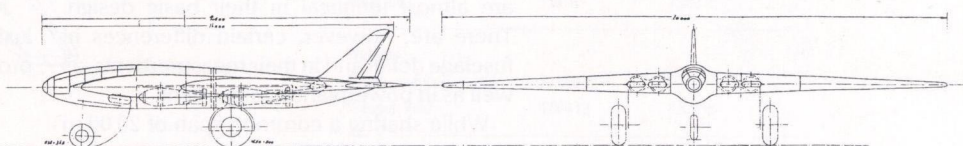
GA drawing of the Messerschmitt P 1107, drawing number IX-122.
