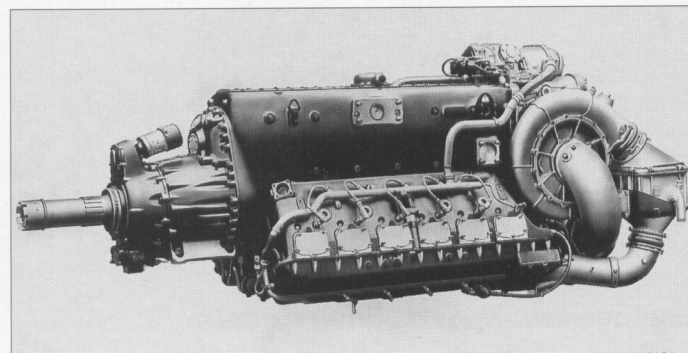
Daimler-Benz DB 627B. 2,000 hp 12-cylinder in-line engine with two-stage supercharger and charge cooling. A further development of the DB 603G.
