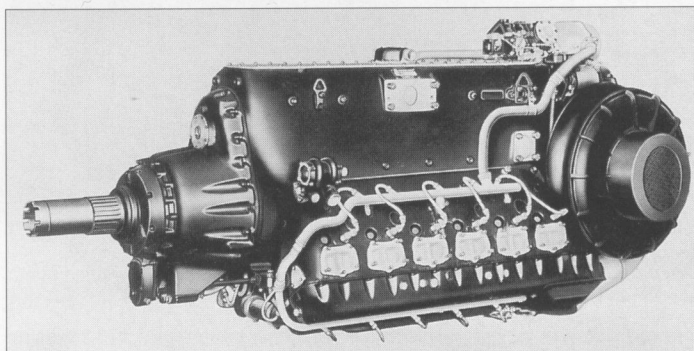
Daimler-Benz DB 605 ASB. 1,850 hp 12-cylinder injection engine with single-stage special supercharger; a high-altitude engine which was to power various bomber projects.
