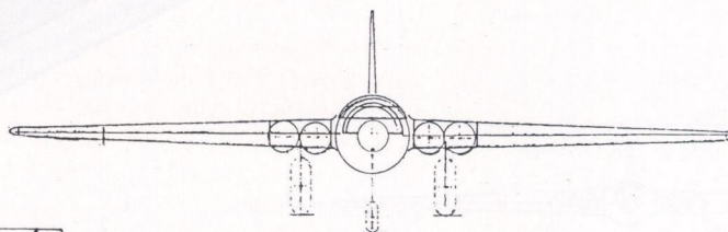
GA drawing of the Messerschmitt P 1108/II, drawing number IX-123.
