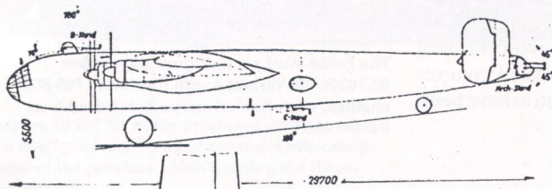
GA drawing of the Focke-Wulf project, drawing number 03.10206-20, the variant with six DB 9-603.
