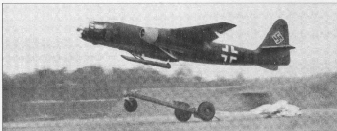
Arado Ar 234A at moment of take-off and release of trolley. The trolley is falling back to earth and the drag chute is starting to open.
