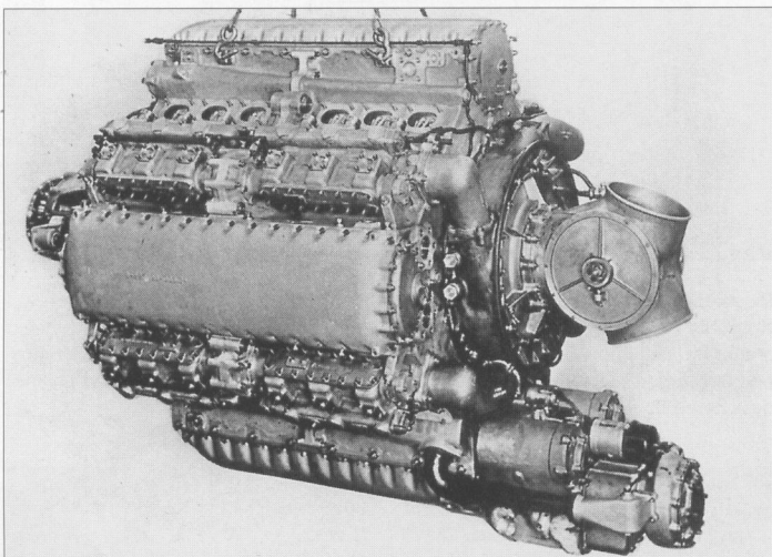
Junkers Jumo 224. 4,000 hp opposed-piston diesel engine with single-stage exhaust gas turbocharger. Driving contra-rotating propellers, this engine was to be fitted in large flying boats operating in strategic roles.
