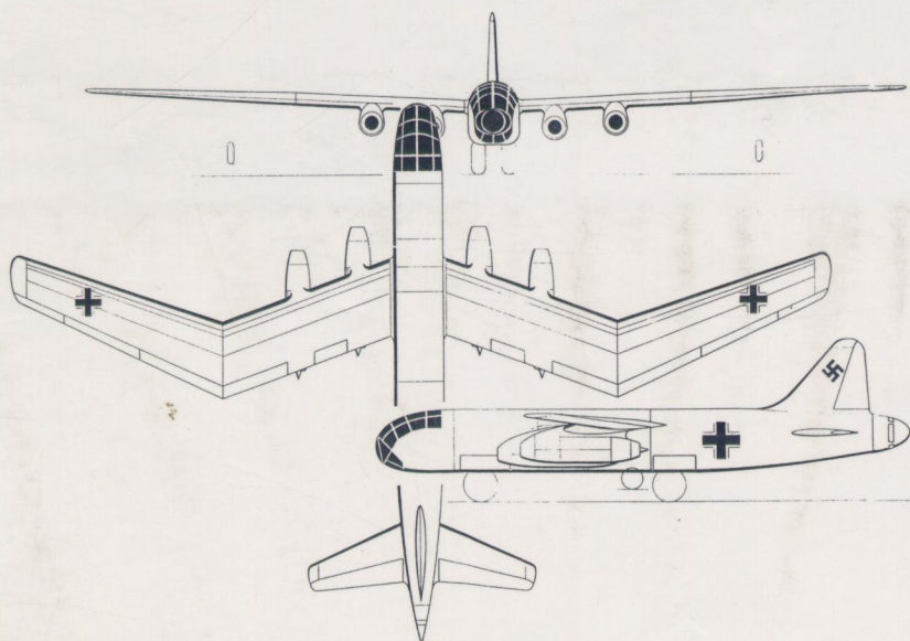
GA drawing of the Blohm & Voss P 188.01 heavy jet bomber, with its noteworthy variable-incidence wing.
