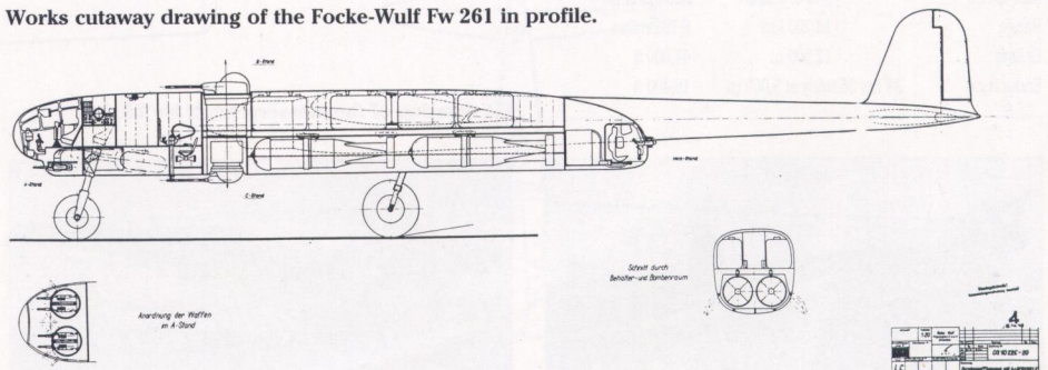
Works cutaway drawing of the Focke-Wulf Fw 261 in profile.
