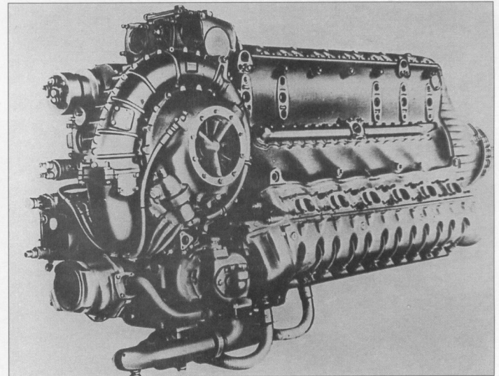
Junkers Jumo 213E. 2,100 hp 12-cylinder high-altitude engine with two-stage supercharger. The Jumo 213 was a masterpiece of German aerodynamic development. A special version, comprising two Jumo 213s coupled in tandem, produced 5,000 hp. This large powerplant was intended for use in long-distance bombers and large flying boats.
