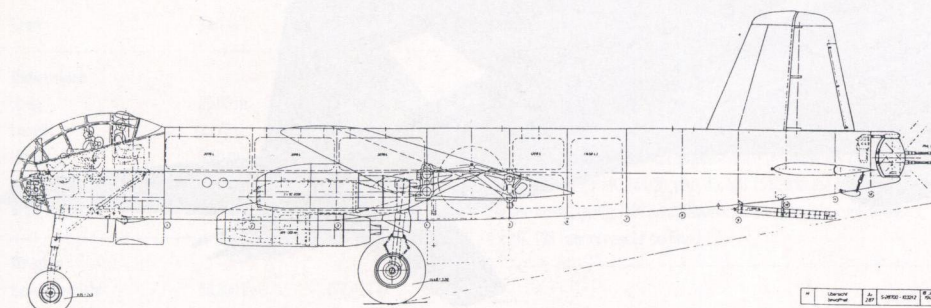
Profile cutaway of the Junkers Ju 287 V3 works drawing.
