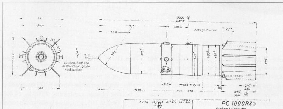
Front and side views of the PC 1000 RS.
