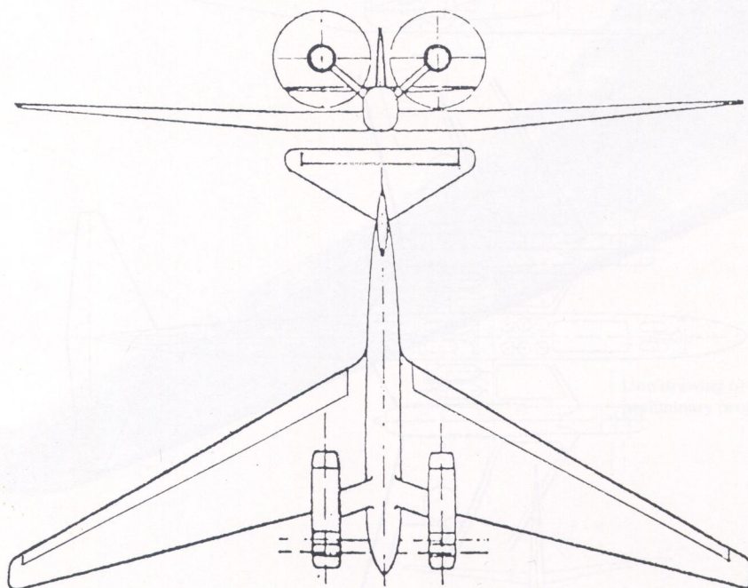
GA drawing of the BMW High-Speed Bomber Project II.
