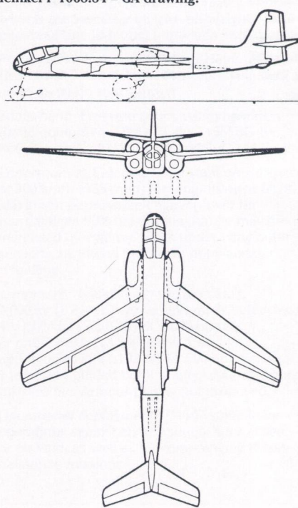
Heinkel P 1068.84 - GA drawing.
