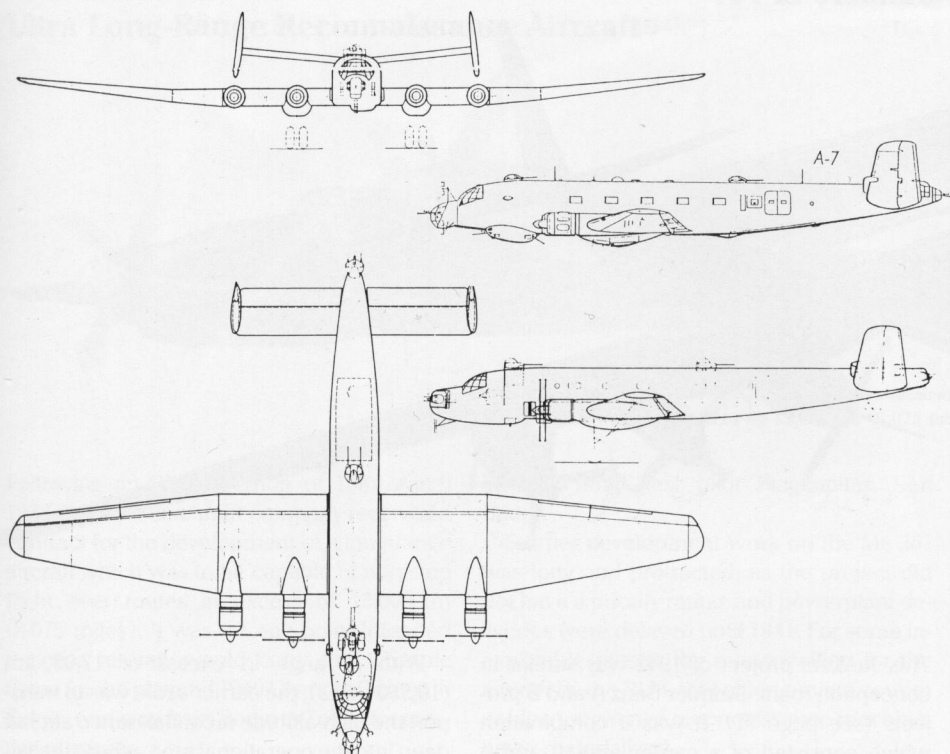
GA drawing of the Junkers Ju 290A-7.
