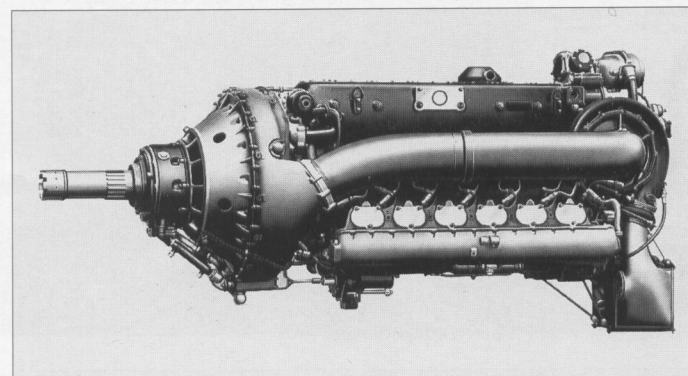
Daimler-Benz DB 628. 1,600 hp 12-cylinder high-altitude engine with two-stage large supercharger.
