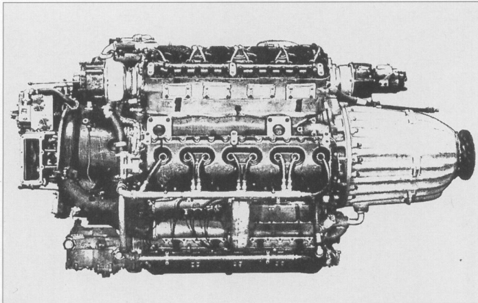
Junkers Jumo 222. 2,500 hp 24-cylinder liquid-cooled multi-row radial engine designed to power the projects developed under the Bomber-B Programme.
