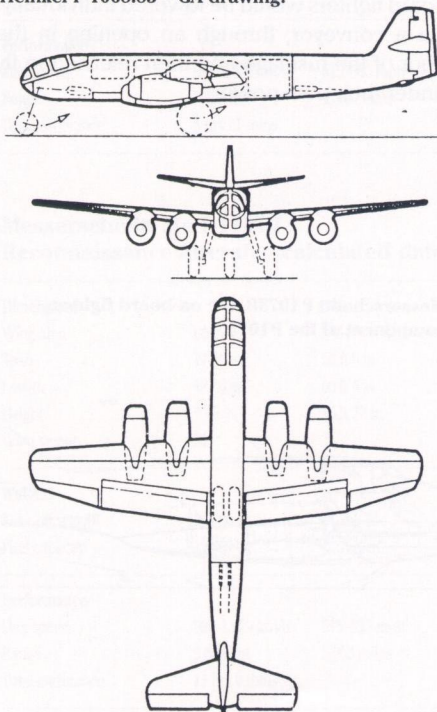
Heinkel P 1068.83 - GA drawing.
