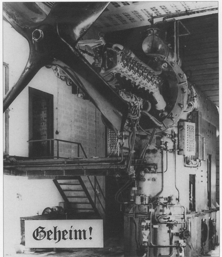
Deutz DZ 710. 3,100 hp 16-cylinder two-stroke engine developed by Klöckner-Humboldt Deutz AG. With fuel injection and exhaust gas turbocharging, this was one of the most powerful piston engines intended for use in various long-distance bomber projects. A further development as a 6,000 hp 32-cylinder coupled engine, designated the DZ 720, was to have powered large flying boats.
