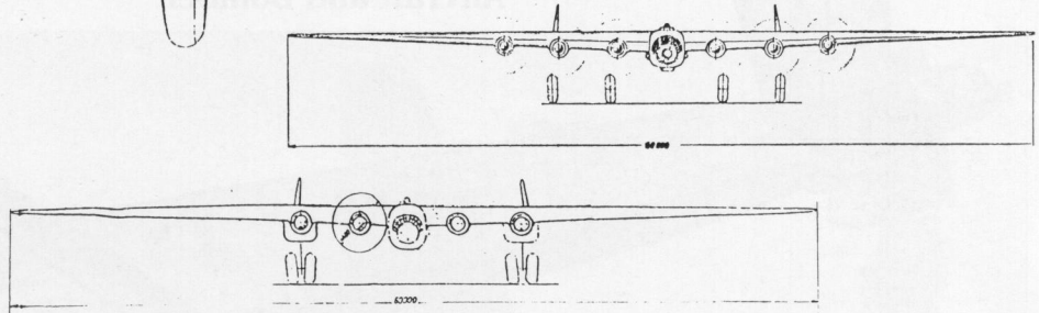
GA drawing of the Focke-Wulf project, drawing number 03.10206-27, with six Junkers Jumo 9-222 engines.
