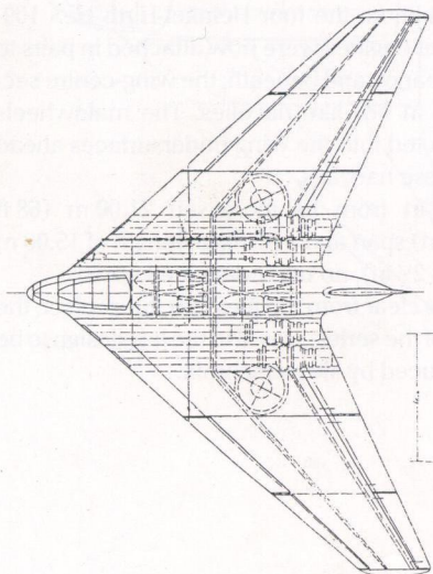
GA drawing of the Messerschmitt P 1107, drawing number IX-122.
