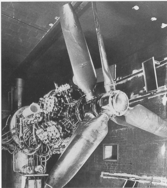
BMW 803. 4,500 hp 28-cylinder liquid-cooled four-row radial engine with boost injection.
