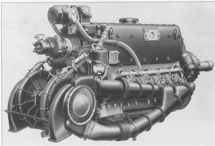
Daimler-Benz DB 623. 2,300 hp 12-cylinder high-altitude engine with turbocharger and charge cooling.
