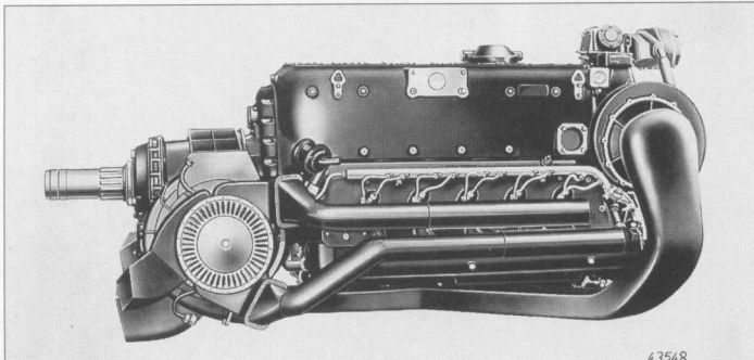
Daimler-Benz DB 621. 1,620 hp 12-cylinder high-altitude engine, developed from the DB 605 with two exhaust gas turbochargers.
