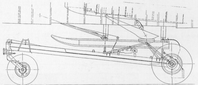
Schematic of the two-wheel take-off trolley used by the Arado Ar 234A-2.
