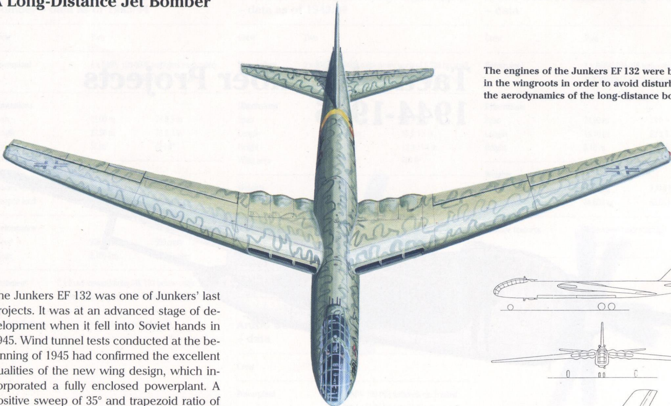
GA drawing of the Junkers EF 132.
