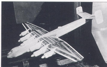
Model of the Tank Ta 400 in the wind tunnel.
