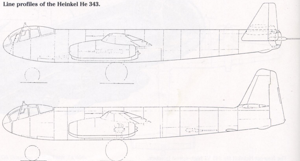
Line profiles of the Heinkel He 343.
