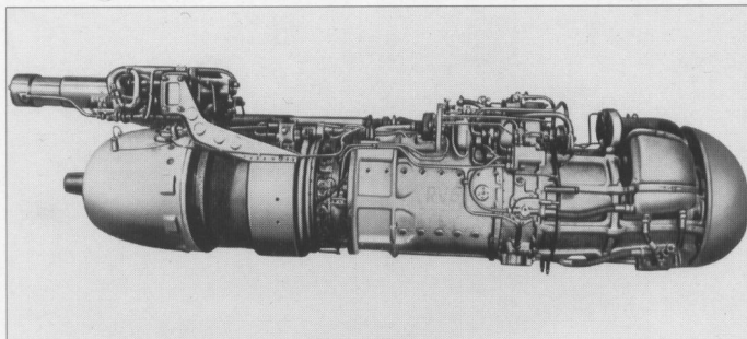
BMW 109-003R. A combination powerplant consisting of a BMW 109-003 turbojet plus a BMW 109-718 liquid fuel rocket engine, delivering 1,250 kg (2,755 lb) static thrust, mounted on a bearer above the jet engine's exhaust pipe. This combination was to have been used on tactical bomber projects.
