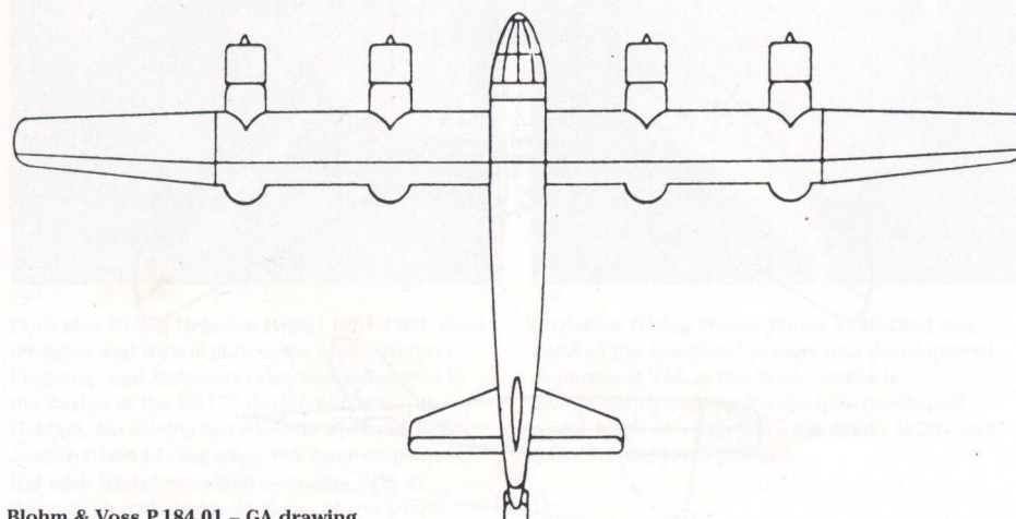
Blohm & Voss P 184.01 – GA drawing.
