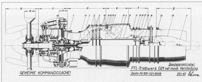
Daimler Benz DB 109-021. 3,300 hp shaft output turboprop version of the Heinkel-Hirth HeS 109-011 jet engine, delivered 1,100 kg (2,424 lb) additional thrust.
