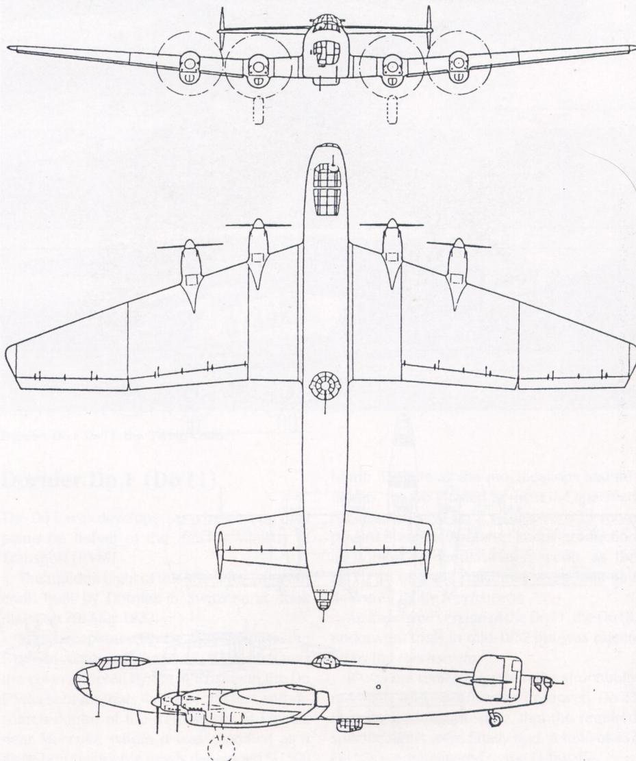
Junkers Ju 89 V1 – GA drawing.
