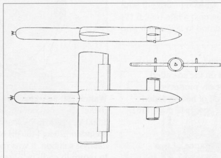
Schematic of the L 11 'Schneewittchen'.
