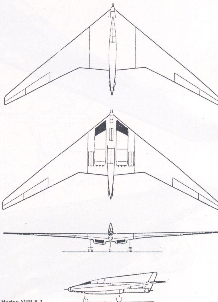
GA drawing of the Horten XVIII B-2.
