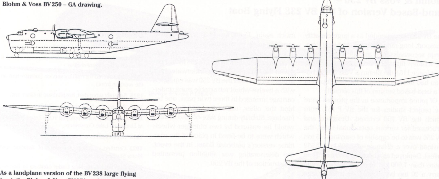
Blohm & Voss BV 250 – GA drawing.
