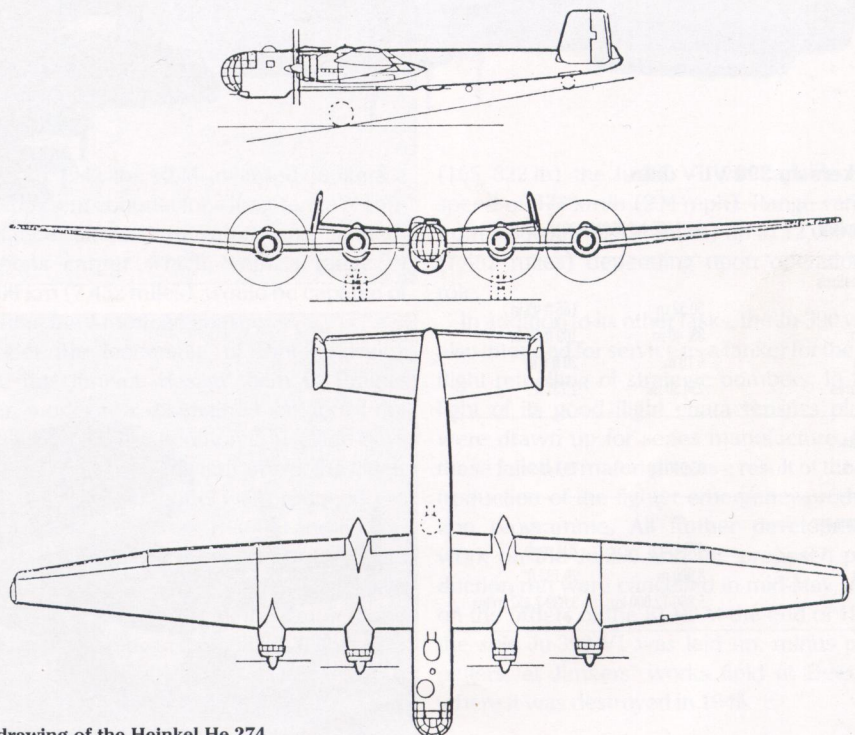
GA drawing of the Heinkel He 274.
