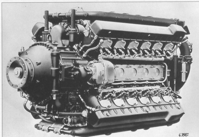
Daimler-Benz DB 604C. 3,500 hp 24-cylinder injection X-engine. After production had begun, the entire DB-604 programme was cancelled on 4th September 1942 upon the orders of the RLM.
