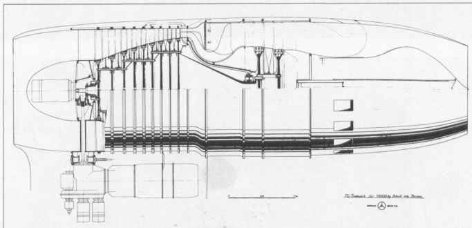
Daimler Benz DB 109-016. 13,000 kg (28,652 lb) static thrust large turbojet. The DB 109-016, developed by Daimler Benz AG in March 1945 and designed for the DB very-high-speed bomber project (Project number 3.10 256-05), was at that time the most powerful turbojet engine in the world. With a length of 6.70 m (21 ft 9 in) and a diameter of some 2 m (6 ft 7 in), it could have been fitted to only the largest of bomber projects.
