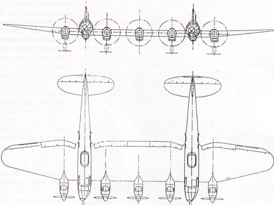
GA drawing of the Heinkel He 111Z-1.
