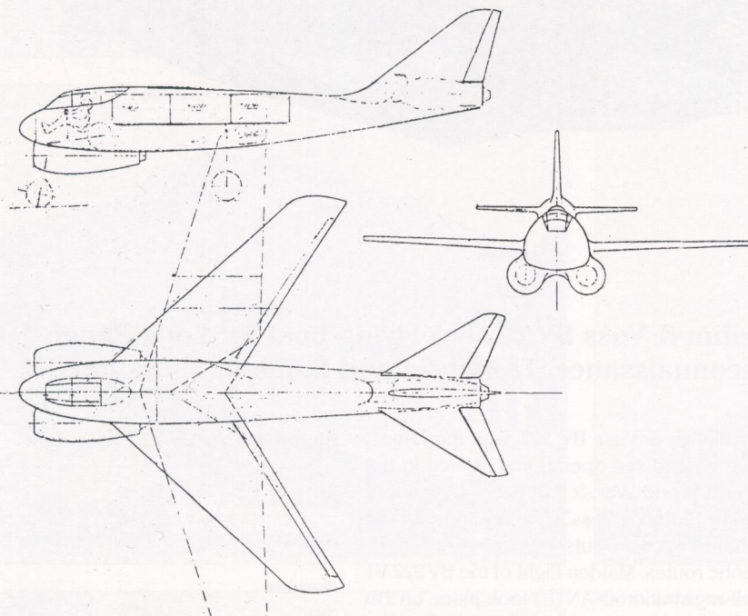
Messerschmitt P 1102/105 – GA drawing.
