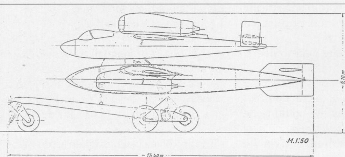
Arado E 377A glide-bomb on the five-wheeled take-off trolley.
