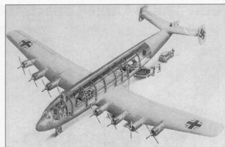
Works impression of the Focke-Wulf large-capacity transport being loaded with wheeled and tracked vehicles.
