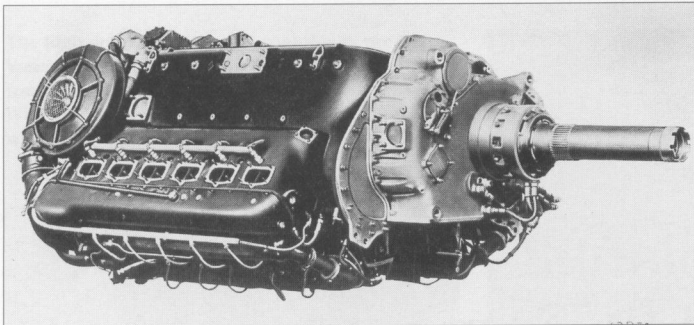
Daimler-Benz DB 613 C-1. 4,000 hp 24-cylinder coupled engine. Construction as DB 606 and DB 610; comprising 2 x DB 603 E/Gs.
