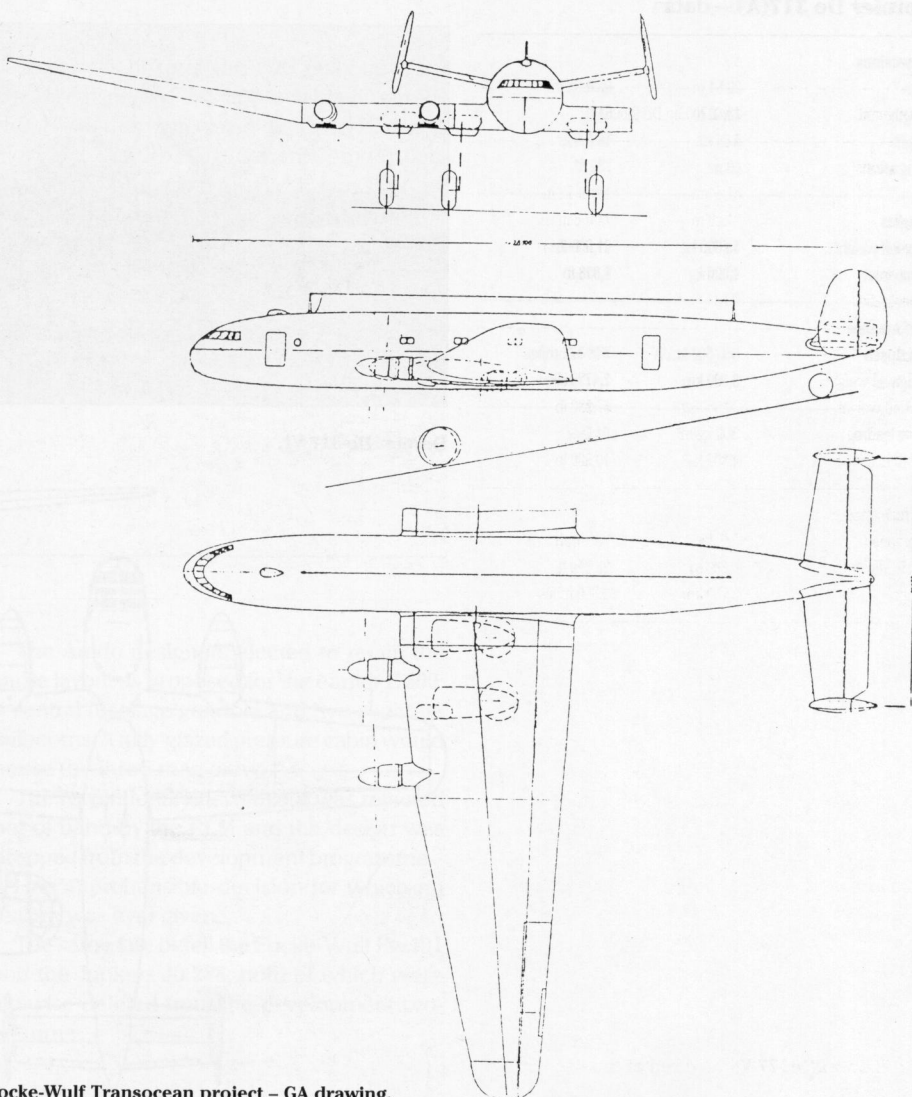
Focke-Wulf Transocean project – GA drawing.
