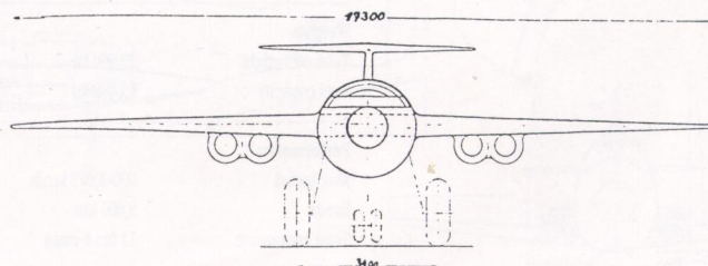
GA drawing of the Messerschmitt P 1107/I.
