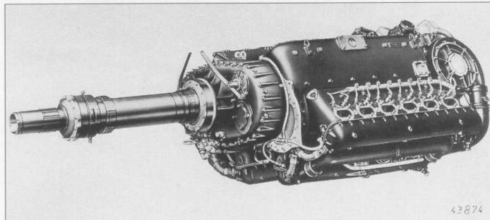
Daimler-Benz DB 606B. 2,700 hp 24-cylinder coupled, or 'double', engine comprising 2 x DB 601Es, which was used to power the Heinkel He 177.
