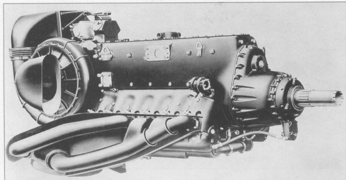
Daimler-Benz DB 624A. 1,900 hp 12-cylinder high altitude engine with exhaust gas turbocharger.
