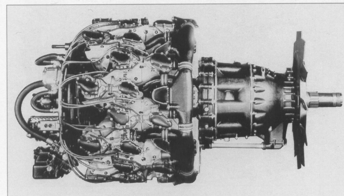
BMW 802. 2,800 hp 18-cylinder twin-row radial engine with exhaust gas turbocharger, intended to power various bomber projects.
