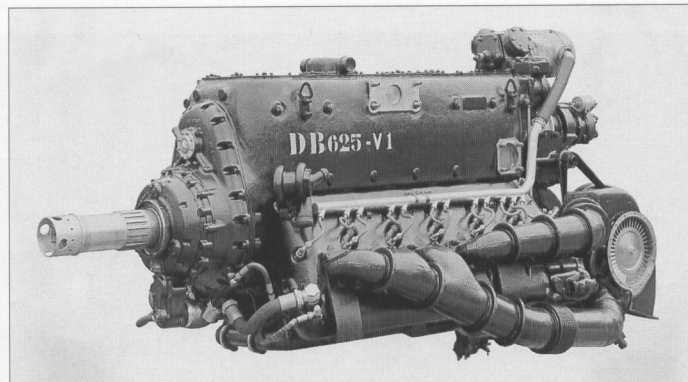
Daimler-Benz DB 625C. 1,755 hp further development of the DB 605D with exhaust gas turbocharger.
