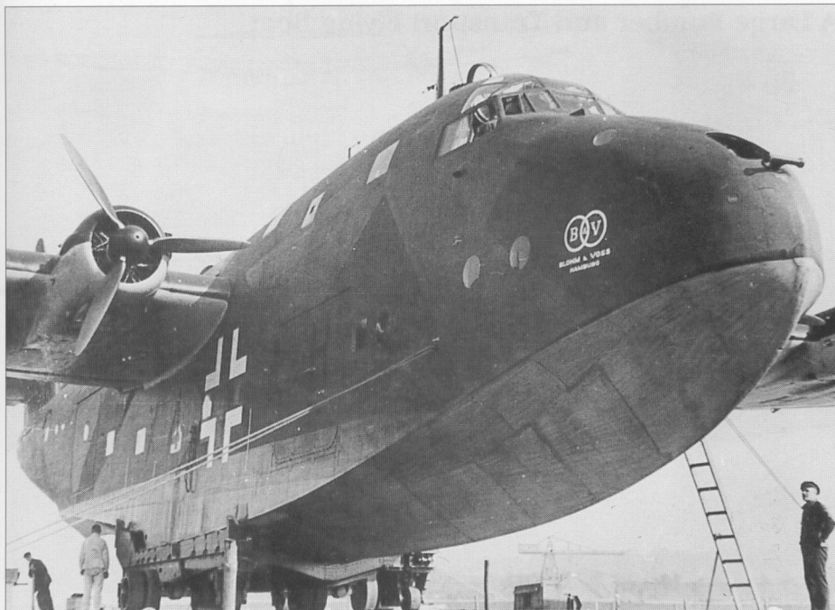
Three-quarter frontal views of the mighty Blohm & Voss BV 222. The flowing lines of the hull are clearly apparent.
