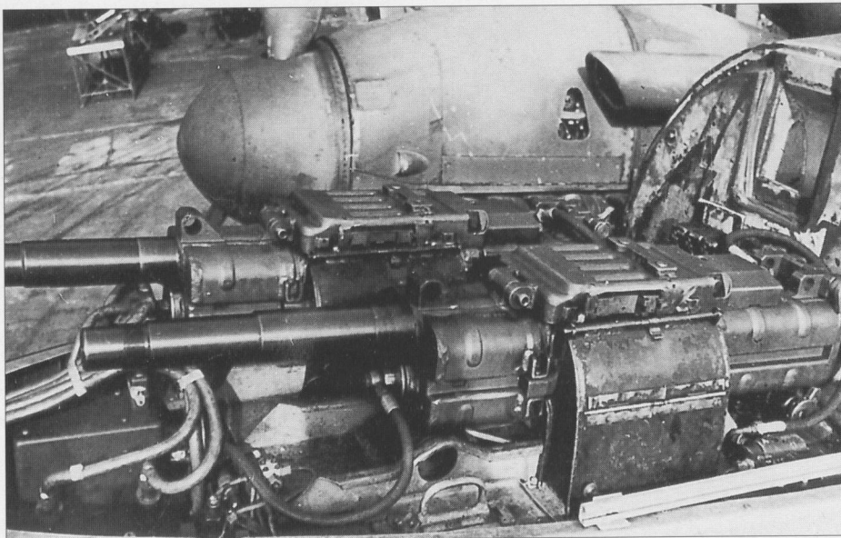
MK 108 cannon in the nose of a Me 110G night-fighter.
