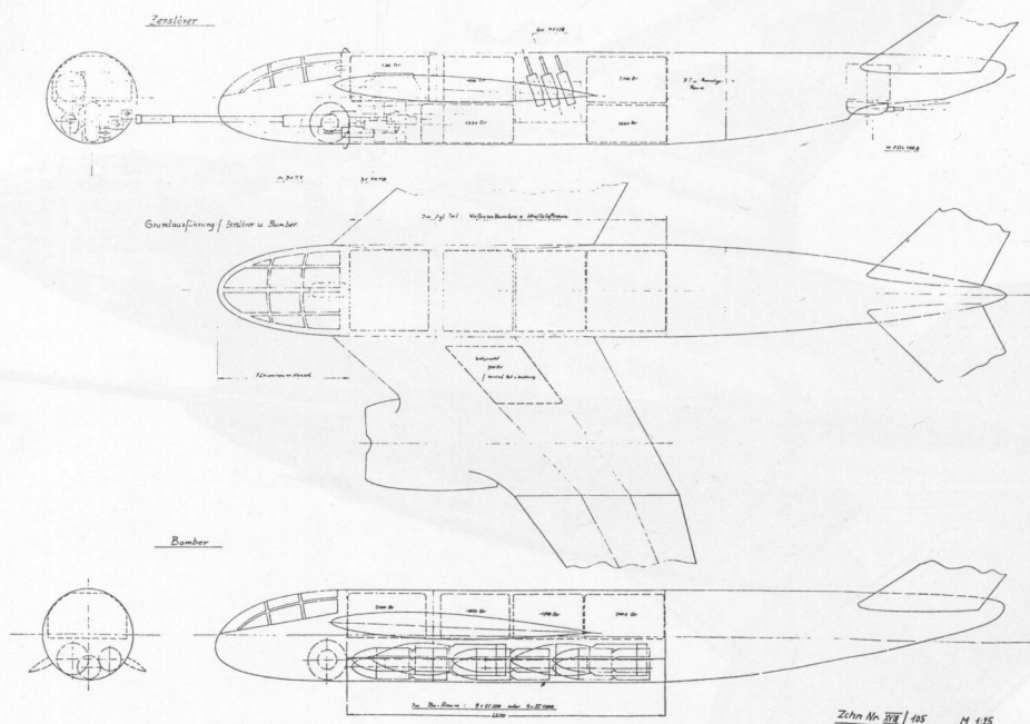
Messerschmitt P 1101/105 – GA drawing.
