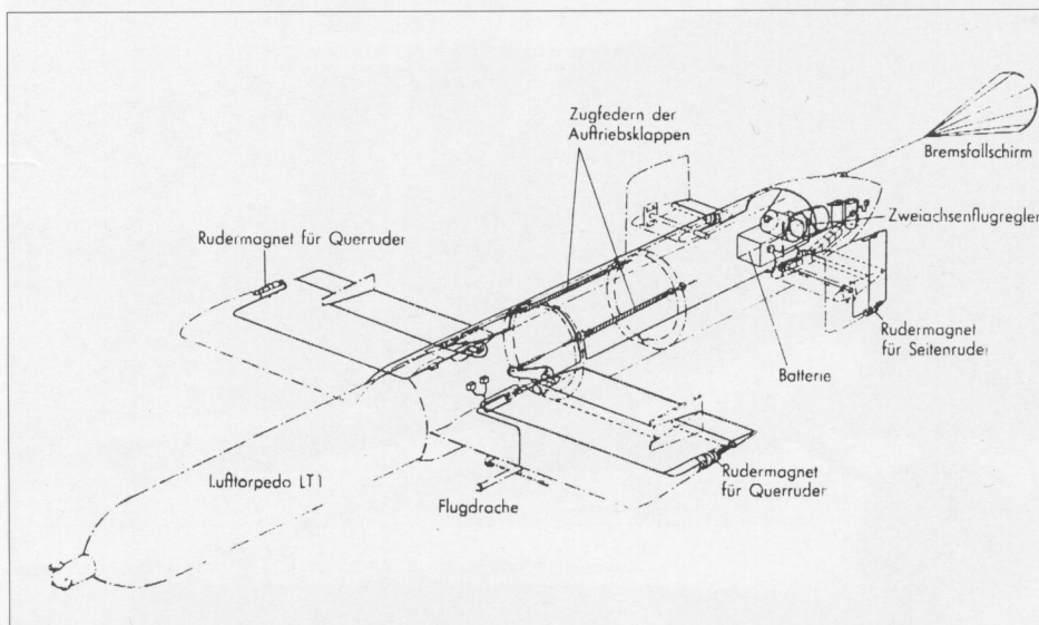
GA drawing of the L 11 'Schneewittchen'.
