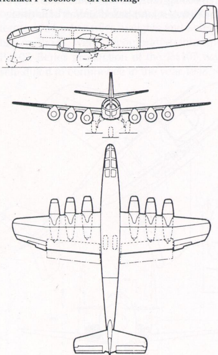
Heinkel P 1068.80 - GA drawing.
