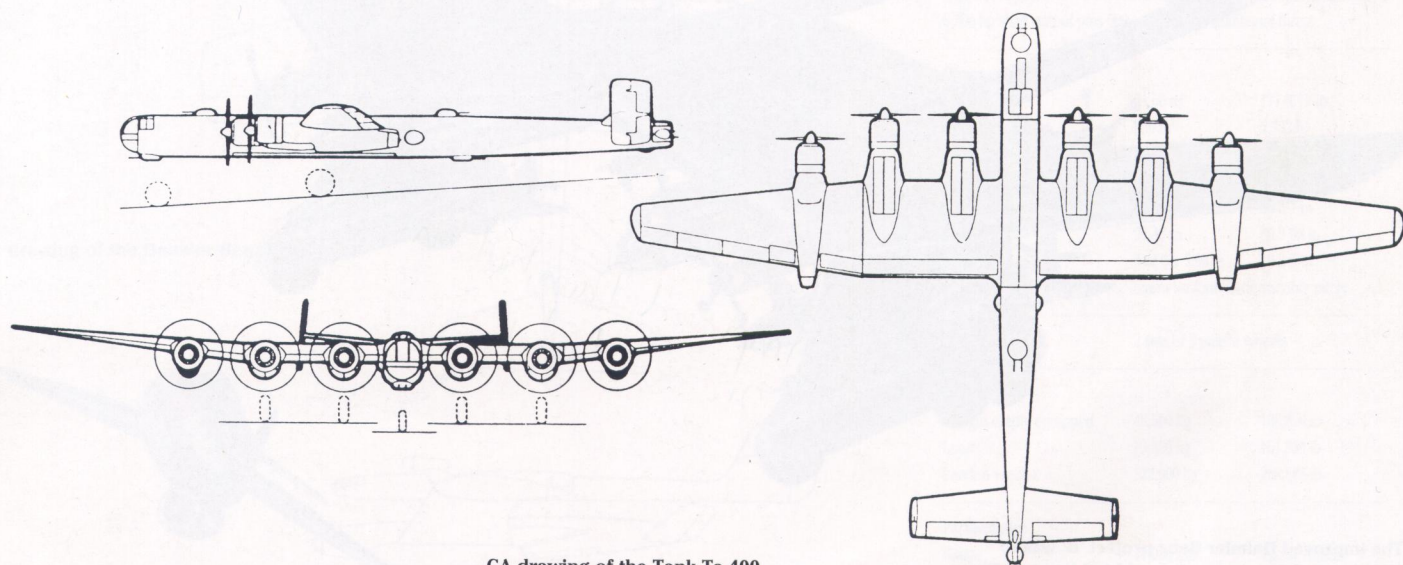
GA drawing of the Tank Ta 400.
