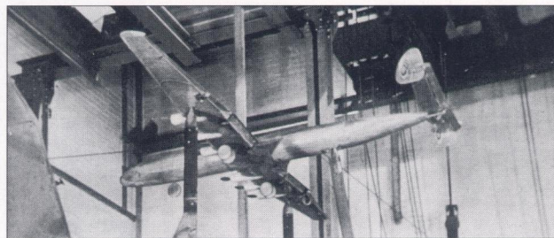
Model of the Junkers EF100 in the wind tunnel.
