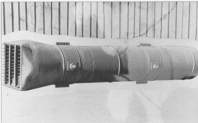
Argus As 109-044. 500-750 kg (1,102-1,653 lb) static thrust pulse-jet. The As 109-044 propulsive duct was a further development of the Argus As 109-014 pulse-jet which powered Fieseler's Fi 103 flying-bomb, better known as the V1. It was intended for use, among other projects, on the Messerschmitt Me 328 parasite fighter.
