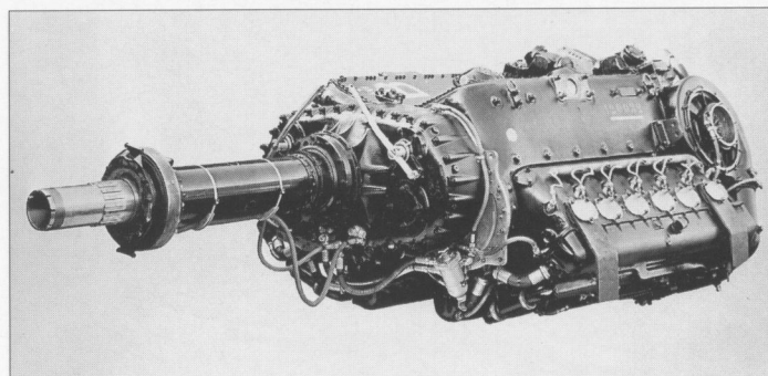
Daimler-Benz DB 610 A-B. 3,000 hp 24-cylinder coupled engine comprising 2 x DB-605s.
