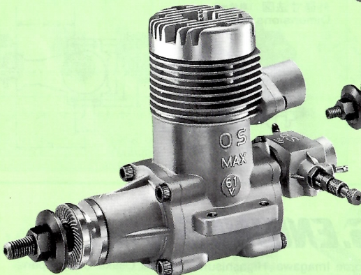
MAX-61VR Æ 10cc FAI CLASS 後方排気 REAR EXHAUST
