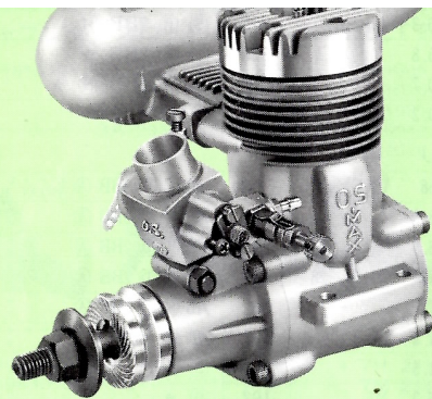
MAX-61FSR Æ MAX-61FSR 10cc FAI CLASS 側方排気 SIDE EXHAUST
