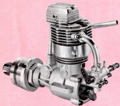
FS-61M
