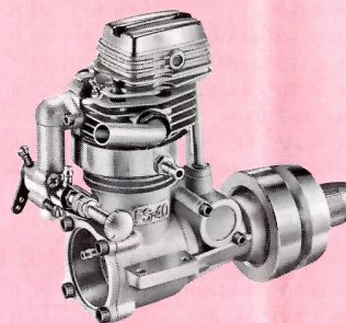
FS-40M
