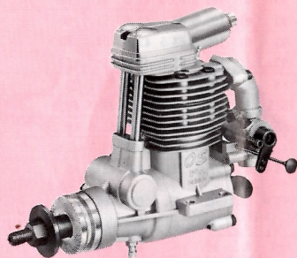
FS-48 SURPASS
