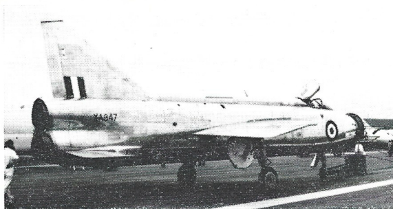
Compare the P.1A with these views of P.1B's XA847 and XG308. The former, photographed at Farnborough in September 1957, was the aerodynamic prototype which took part in trials with the Double Scorpion rocket motor. XG308, seen here the following year, was the second aircraft in the development batch. (Photo: J. M. G. Gradidge)
