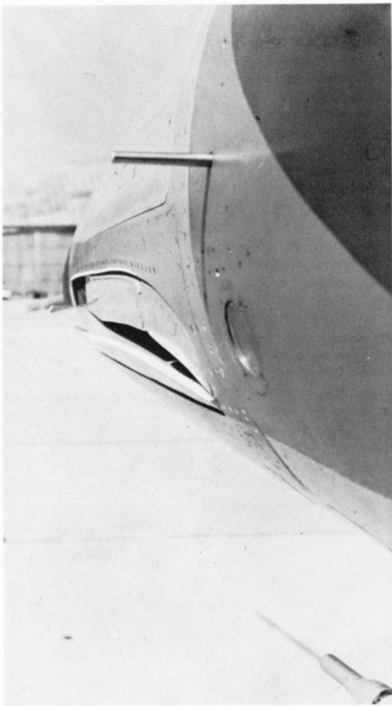
Sequence showing deployment of the retractable foreplanes fitted to a Mirage III.
