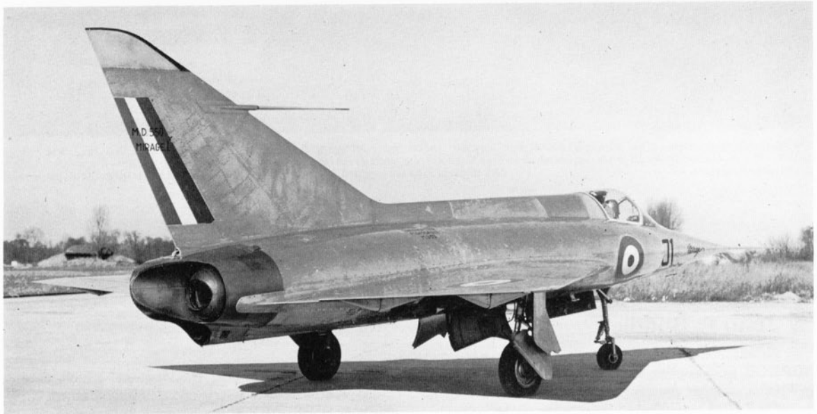
After initial flight trials, the Mirage I-01 was modified and re-engined. Note the redesigned vertical tail surfaces.
